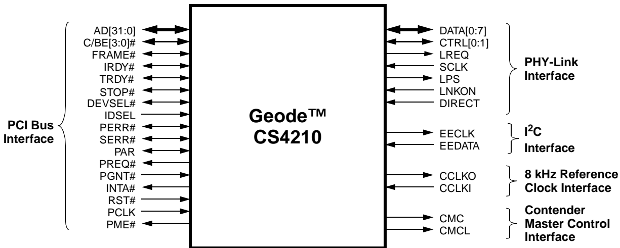
Figure 2-1. Signal Groups
