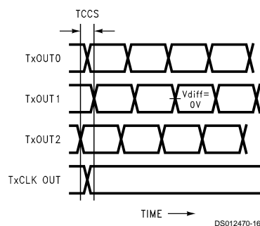
FIGURE 6. DS90CR561 (Transmitter) Channel-to-Channel Skew and Pulse Width
