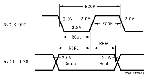
FIGURE 8. DS90CR562 Setup/Hold and High/Low Times
