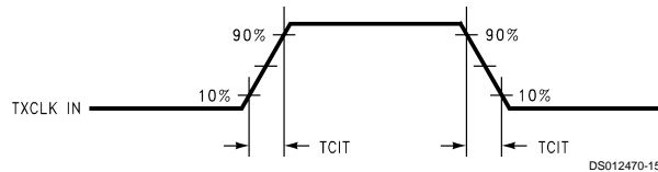
FIGURE 5. DS90CR561 (Transmitter) Input Clock Transition Time
