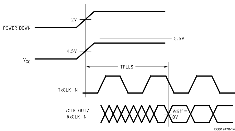
FIGURE 11. DS90CR561 (Transmitter) Phase Lock Loop Set Time
