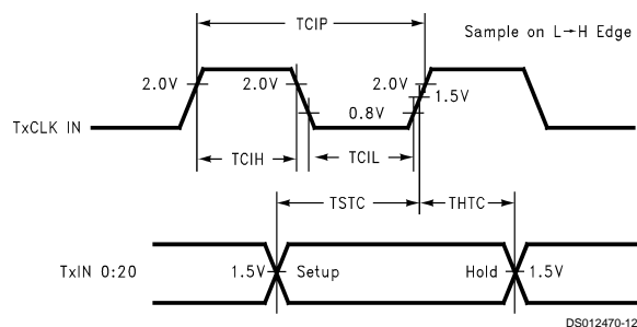
FIGURE 7. DS90CR561 Setup/Hold and High/Low Times
