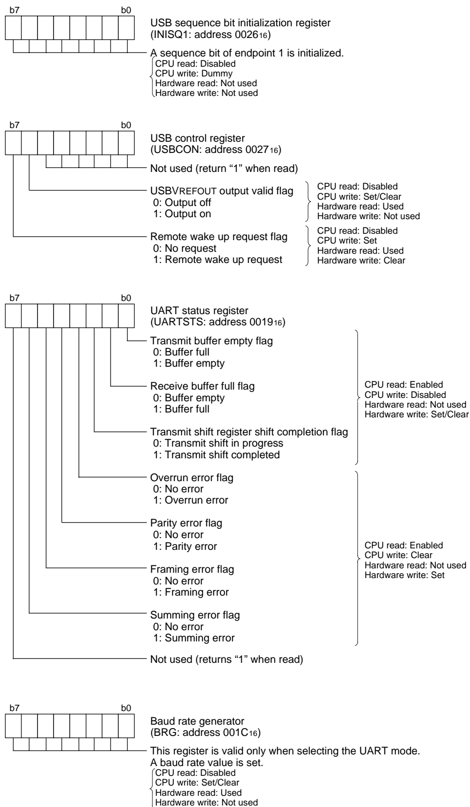
Fig. 29 Structure of serial I/O1-related registers (4)
