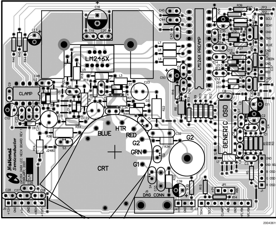
FIGURE 13. LM126X/LM246X Demo Board Layout
