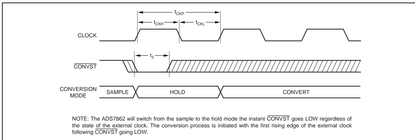
FIGURE 8. Conversion Mode.
