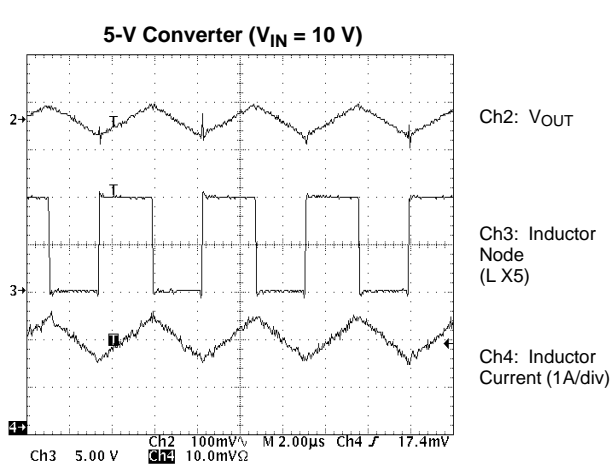
PWM Operation
