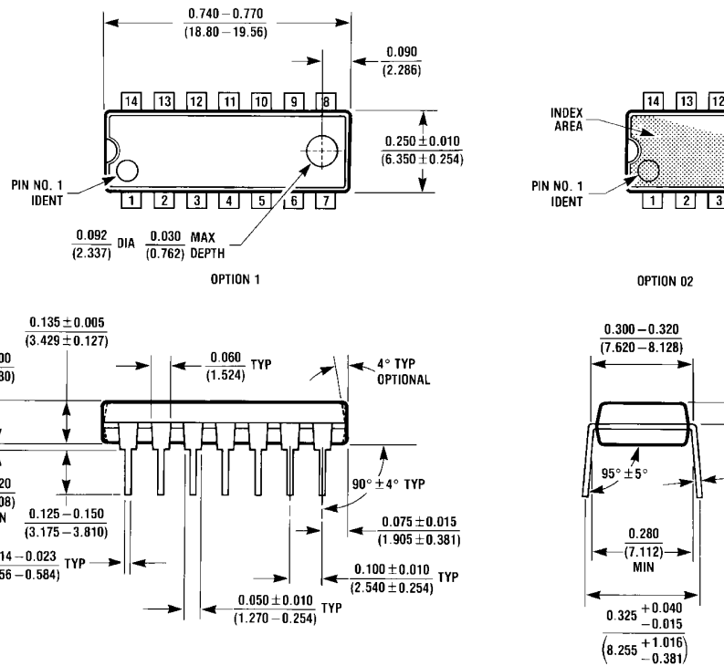
Molded Dual-In-Line Package (N) NS Package Number N14A
