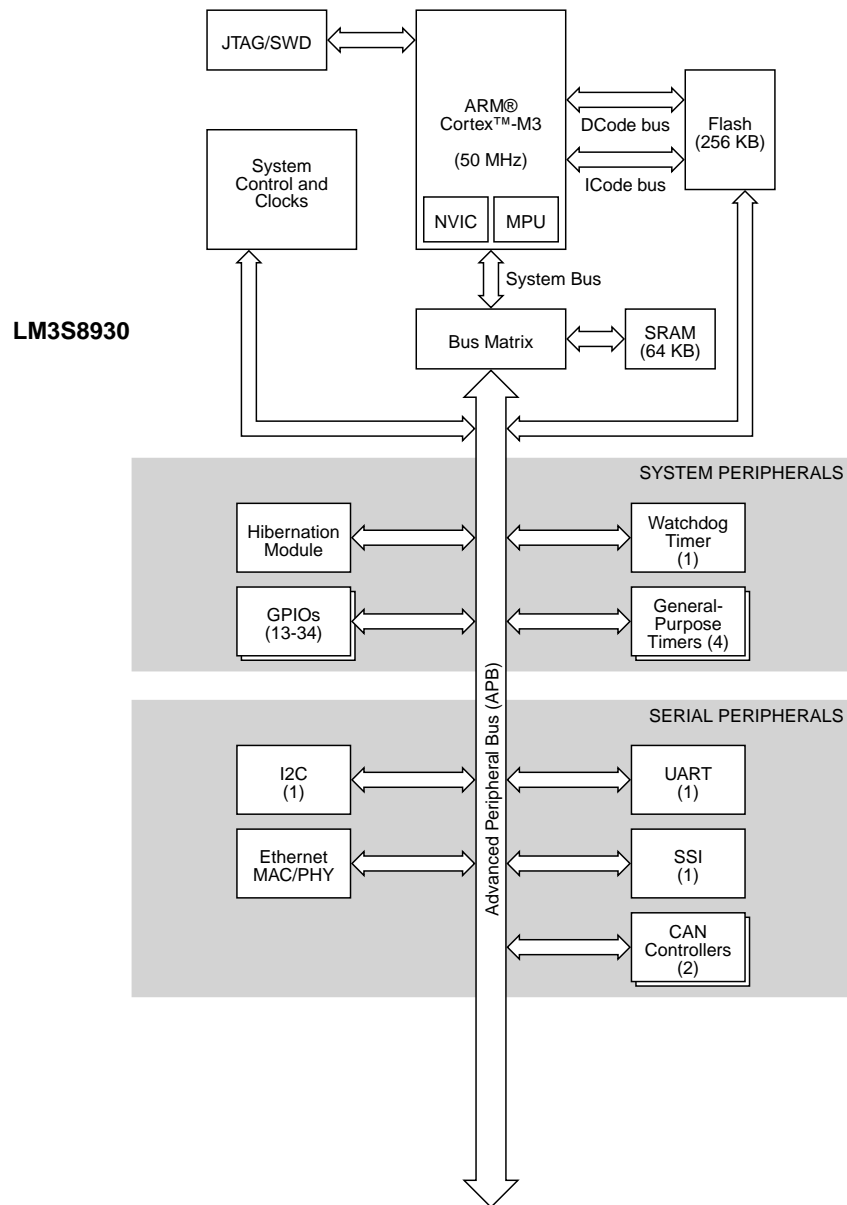
Figure 1-1. Stellaris® LM3S8930 Microcontroller High-Level Block Diagram
