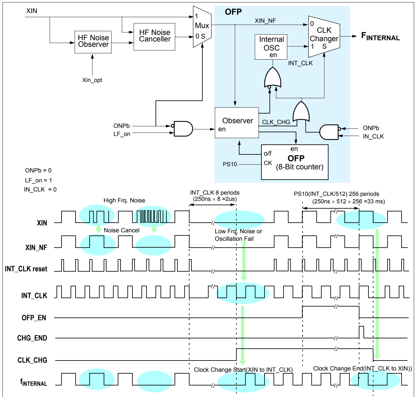
Figure 21-1 Block Diagram of ONP & OFP and Respective Wave Forms
