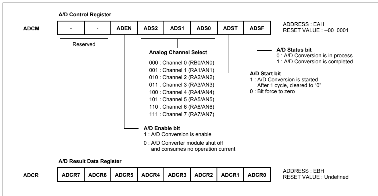
Figure 15-2 A/D Converter Registers
