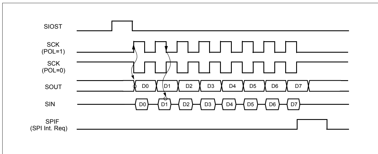
Figure 13-2 SPI Timing Diagram (without SRDY control)
