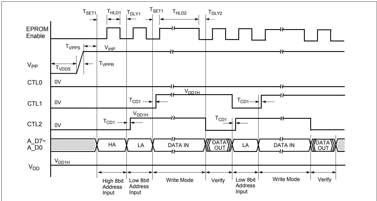
Figure 22-2 Timing Diagram in Program (Write &amp; Verify) Mode
