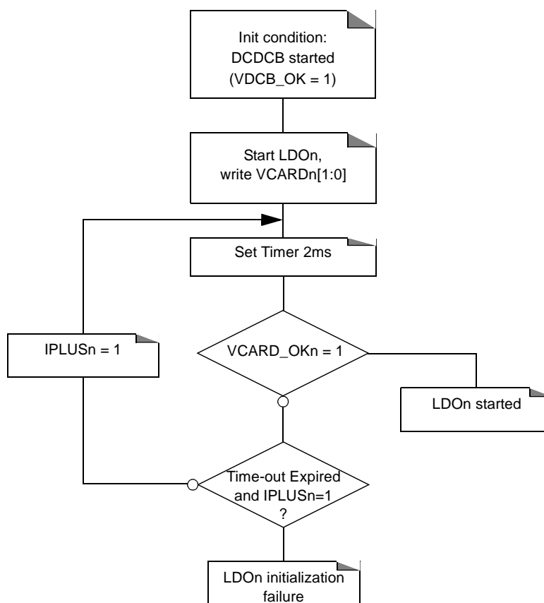
Figure 11. LDO n Initialization Procedure (n = 2, 3, 4, 5)
