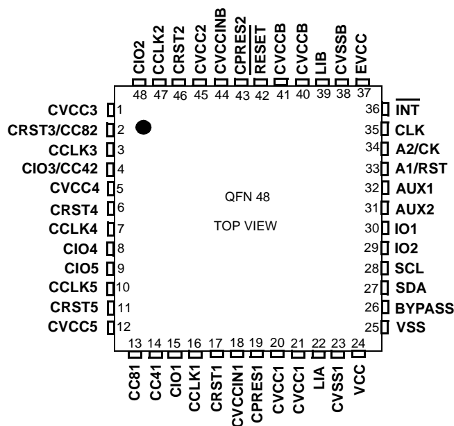
QFN48 Pinout
