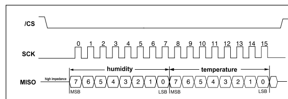
Figure 4 AH31 SPI readout sequence
