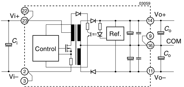
Fig. 2 Dual output converter block diagram
