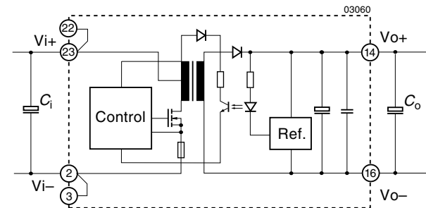
Fig. 1 Single output converter block diagram
