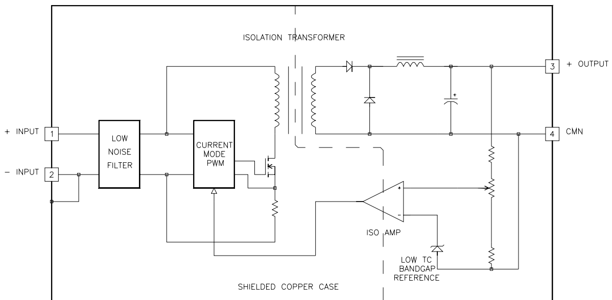
10 Watt NT Single Series Block Diagram
