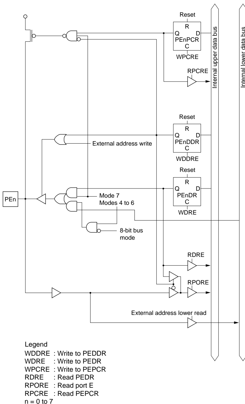
Figure C-24 Port E Block Diagram (Pins PE0 to PE7)
