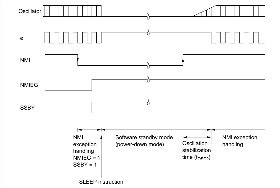
Figure 17-3 Software Standby Mode Application Example
