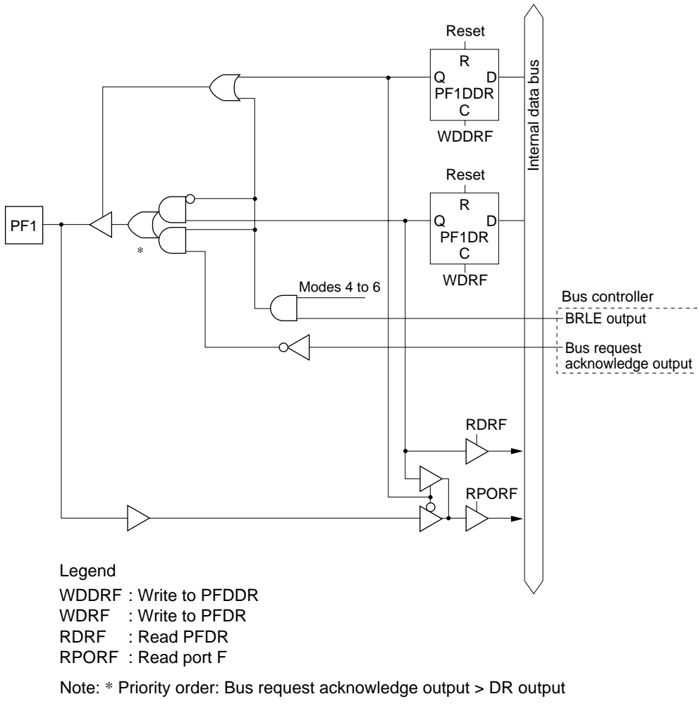
Figure C-26 Port F Block Diagram (Pin PF1)
