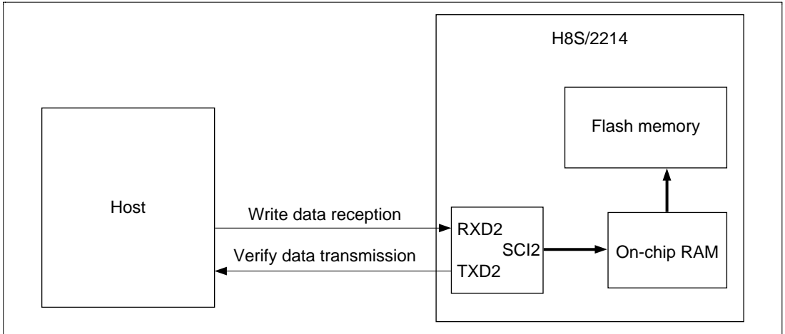
Figure 15-9 System Configuration in Boot Mode
