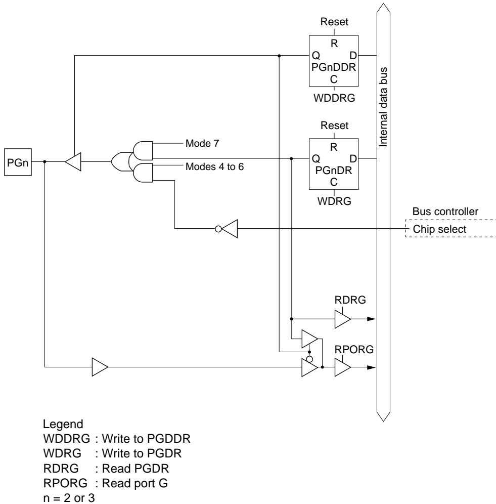
Figure C-33 Port G Block Diagram (Pins PG2 and PG3)
