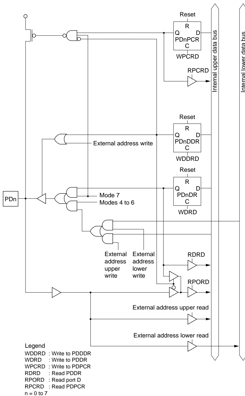
Figure C-23 Port D Block Diagram (Pins PD0 to PD7)
