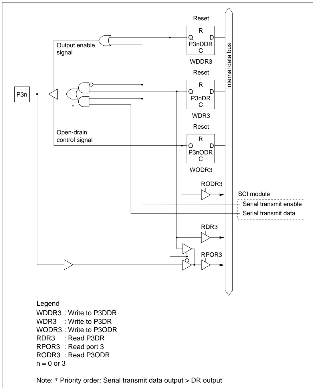
Figure C-5 Port 3 Block Diagram (Pins P30 and P33)
