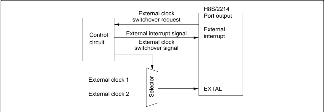
Figure 16-7 Example of External Clock Switching Circuit
