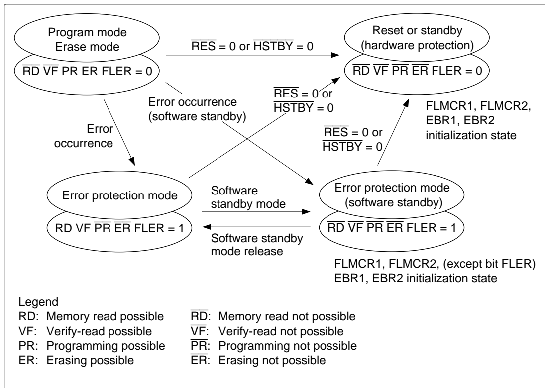
Figure 15-16 Flash Memory State Transitions
