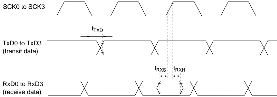
Figure 18-16 SCI Input/Output Timing (Clock Synchronous Mode)
