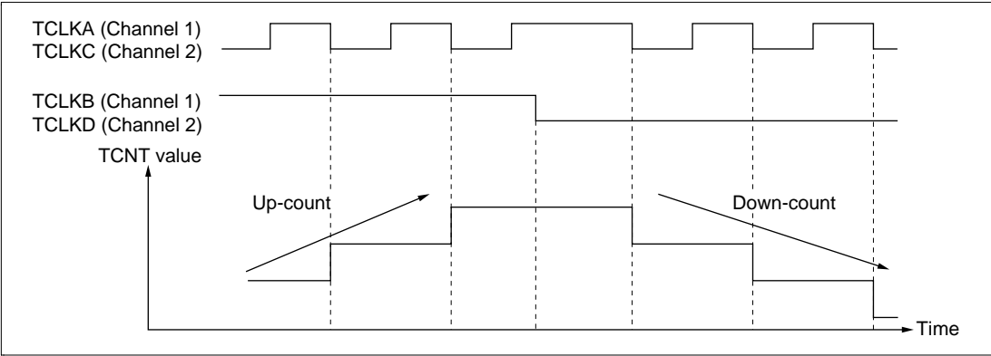
Figure 10-27 Example of Phase Counting Mode 2 Operation
