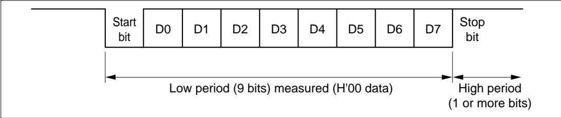
Figure 15-11 Automatic SCI Bit Rate Adjustment
