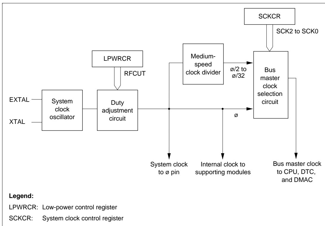
Figure 16-1 Block Diagram of Clock Pulse Generator
