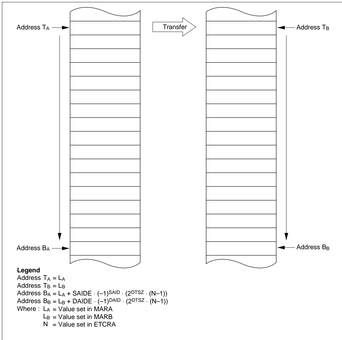
Figure 7-9 Operation in Normal Mode
