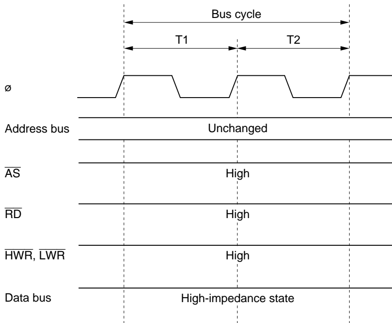
Figure 2-21 Pin States during On-Chip Supporting Module Access
