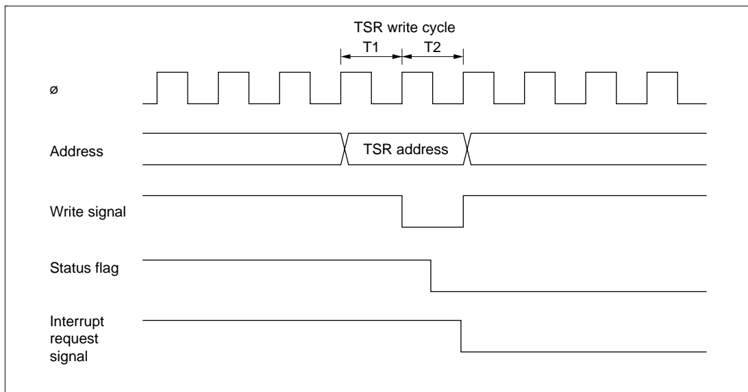
Figure 10-42 Timing for Status Flag Clearing by CPU
