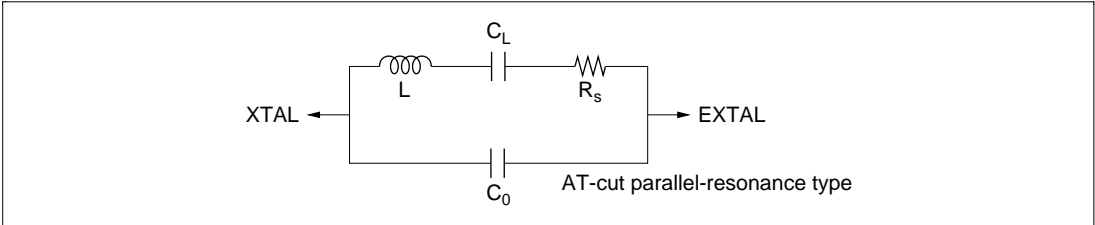
Figure 16-3 Crystal Resonator Equivalent Circuit
