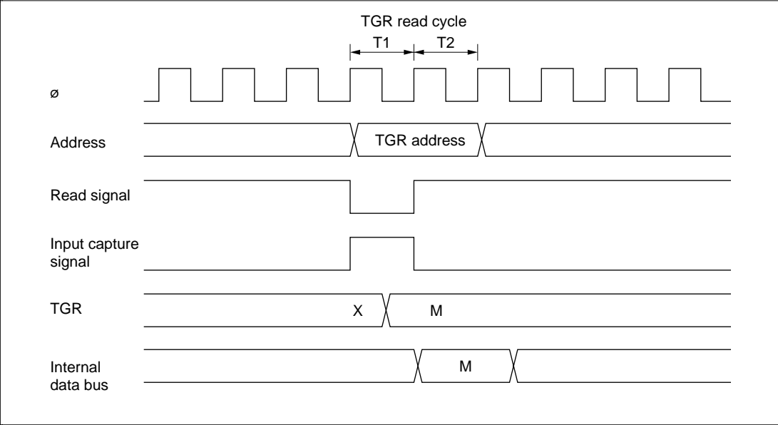
Figure 10-49 Contention between TGR Read and Input Capture
