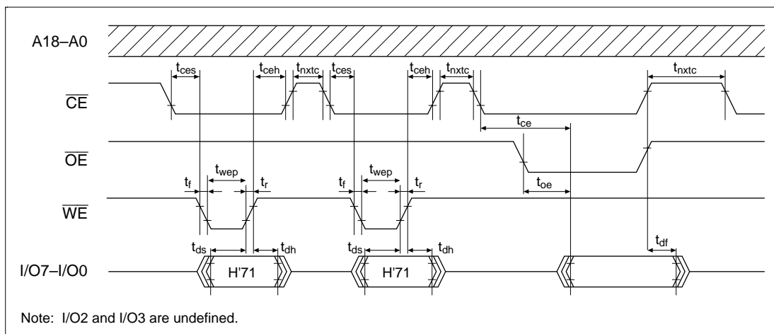
Figure 15-27 Status Read Mode Timing Waveforms
