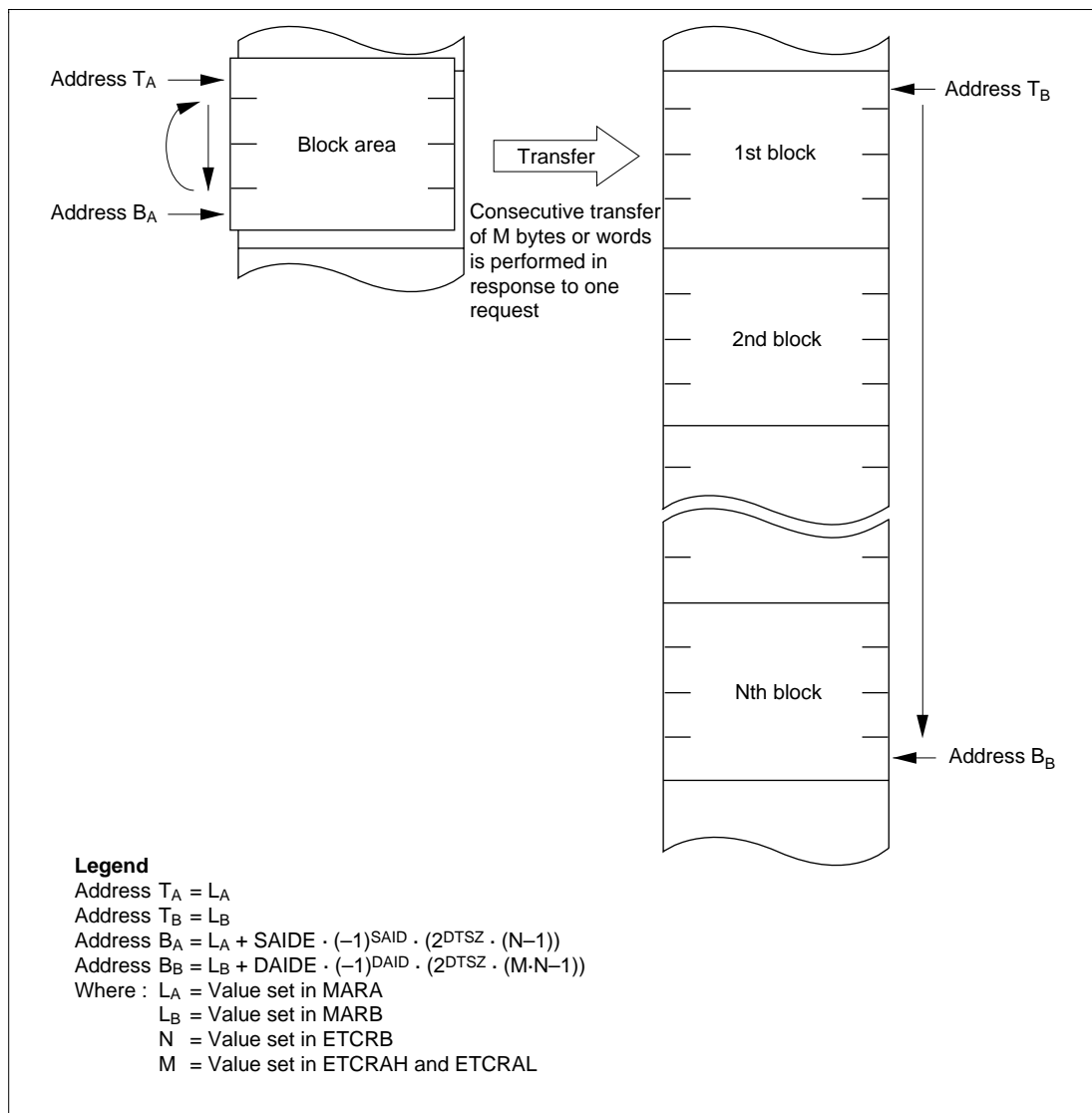
Figure 7-12 Operation in Block Transfer Mode (BLKDIR = 1)
