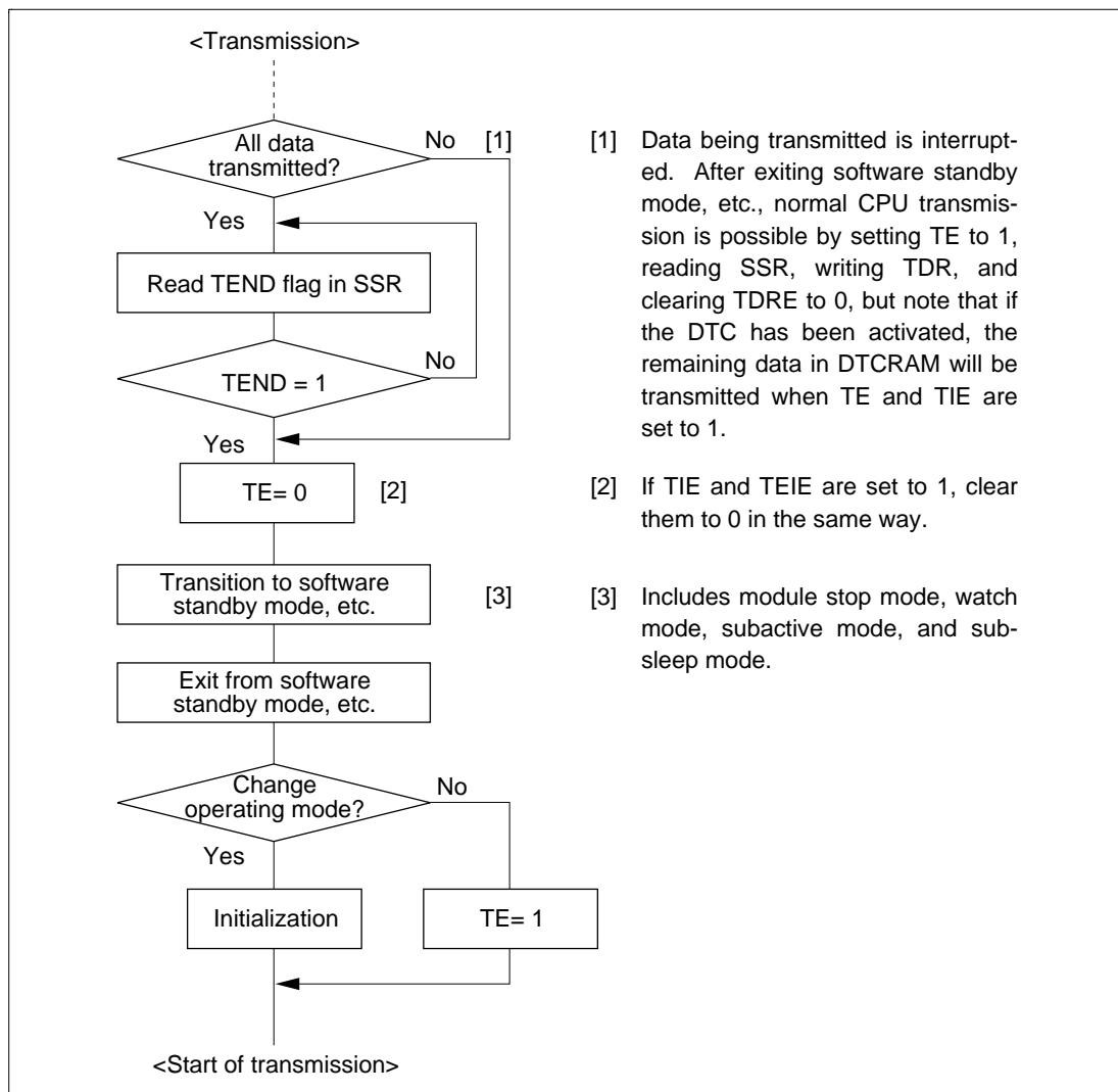
Figure 12-28 Sample Flowchart for Mode Transition during Transmission
