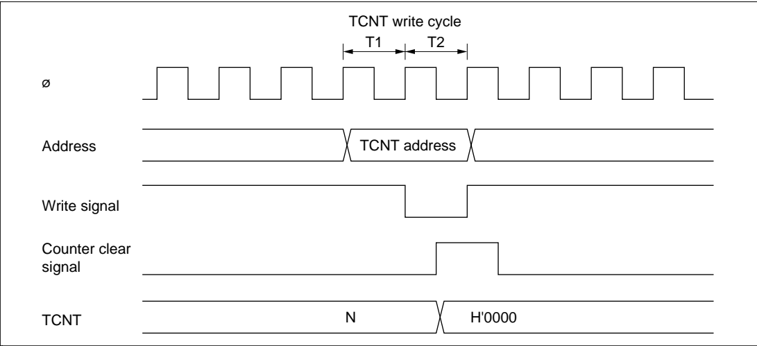
Figure 10-45 Contention between TCNT Write and Clear Operations
