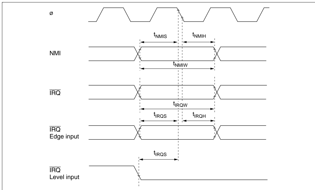
Figure 18-6 Interrupt Input Timing
