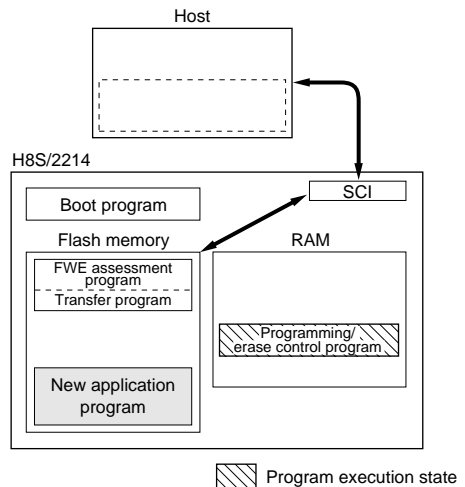
Figure 15-5 User Program Mode
