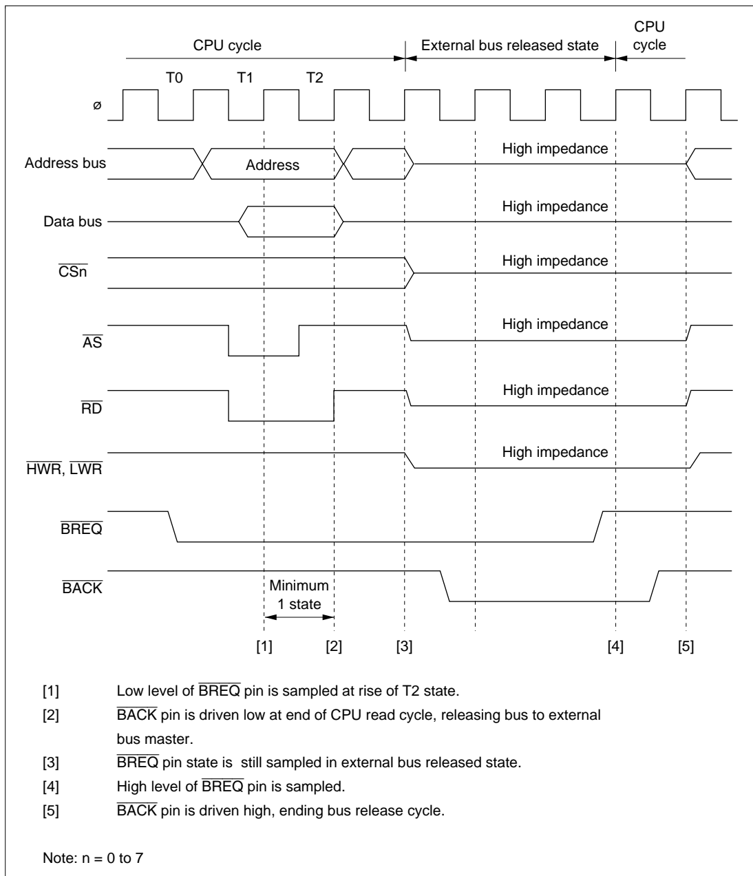
Figure 6-20 Bus-Released State Transition Timing
