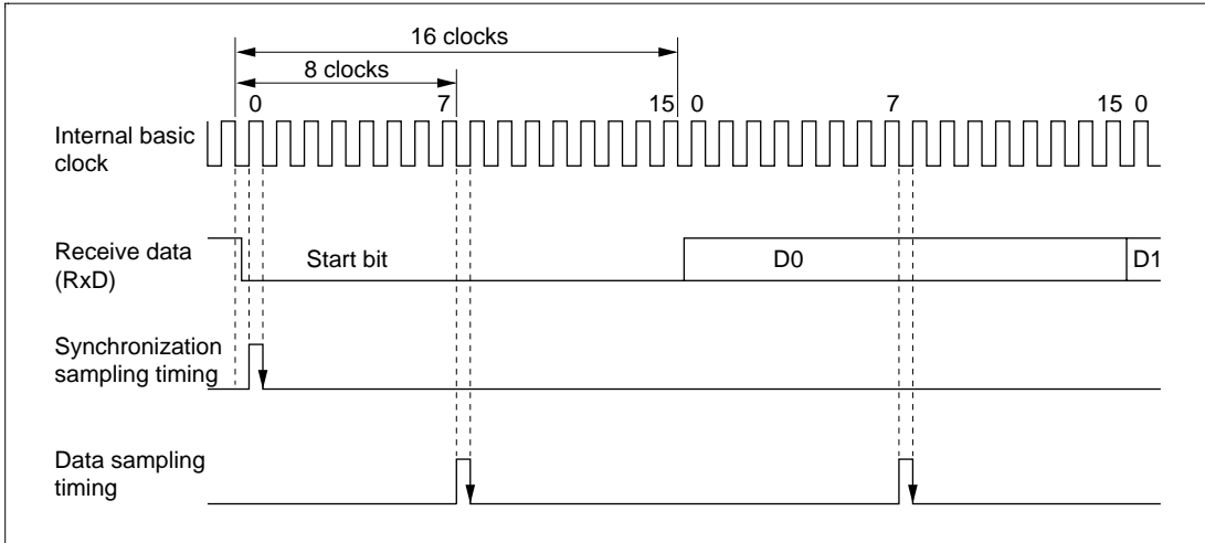
Figure 12-26 Receive Data Sampling Timing in Asynchronous Mode
