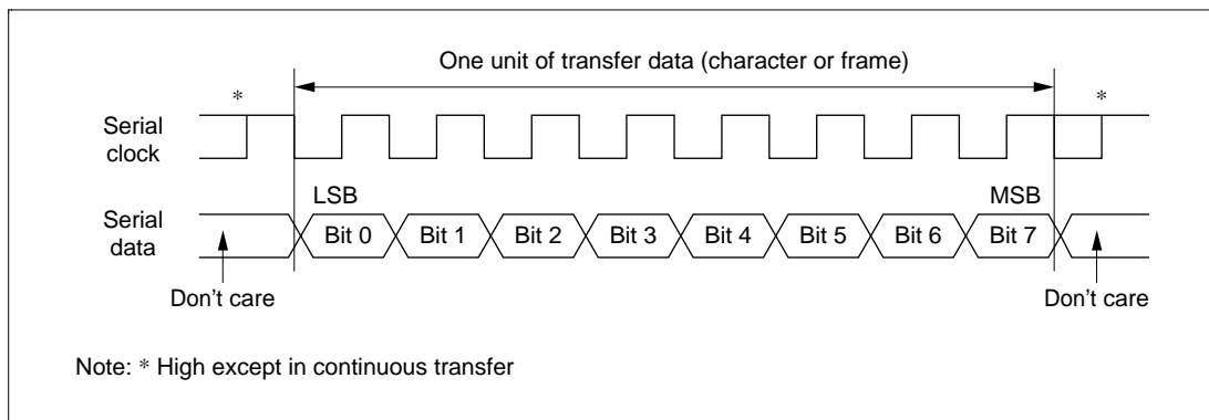
Figure 12-19 Data Format in Synchronous Communication
