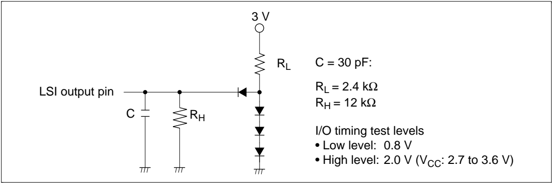
Figure 18-2 Output Load Circuit
