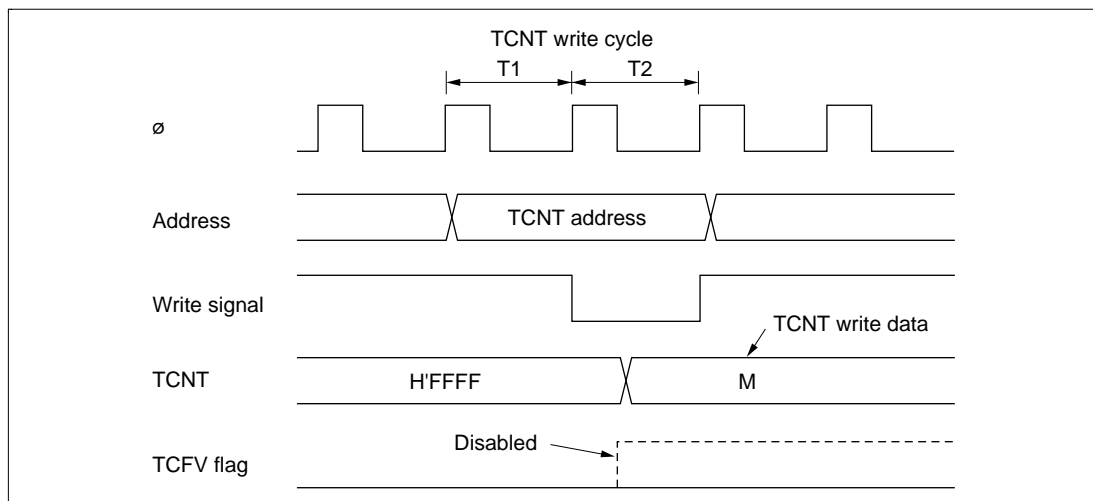
Figure 10-53 Contention between TCNT Write and Overflow
