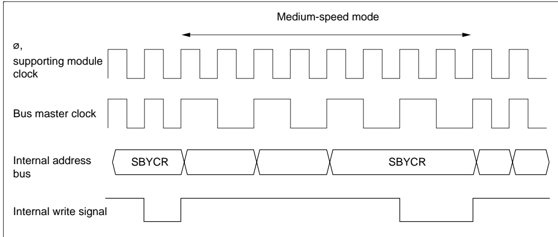
Figure 17-2 Medium-Speed Mode Transition and Clearance Timing
