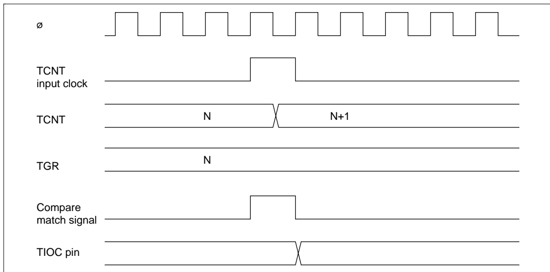
Figure 10-32 Output Compare Output Timing
