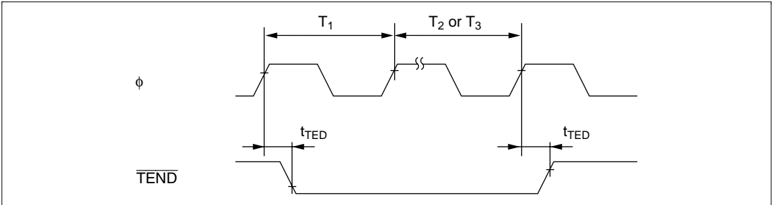
Figure 18-17 DMAC \overline{TEND} Output Timing
