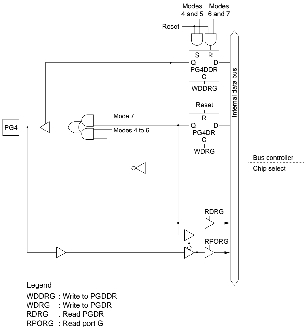
Figure C-34 Port G Block Diagram (Pin PG4)
