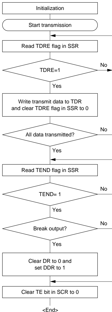
Figure 12-8 Sample Serial Transmission Flowchart
