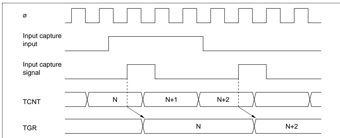
Figure 10-33 Input Capture Input Signal Timing
