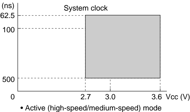
Figure 18-1 Power Supply Voltage and Operating Ranges
