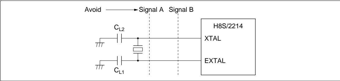
Figure 16-4 Example of Incorrect Board Design
