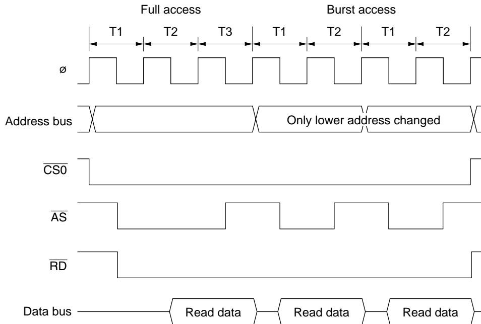
Figure 6-15 Example of Burst ROM Access Timing (When AST0 = BRSTS1 = 1)
