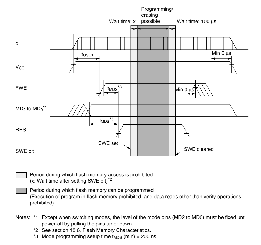
Figure 15-29 Power-On/Off Timing (Boot Mode)
