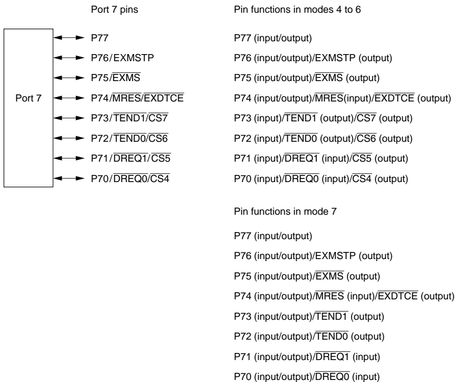
Figure 9-4 Port 7 Pin Functions
