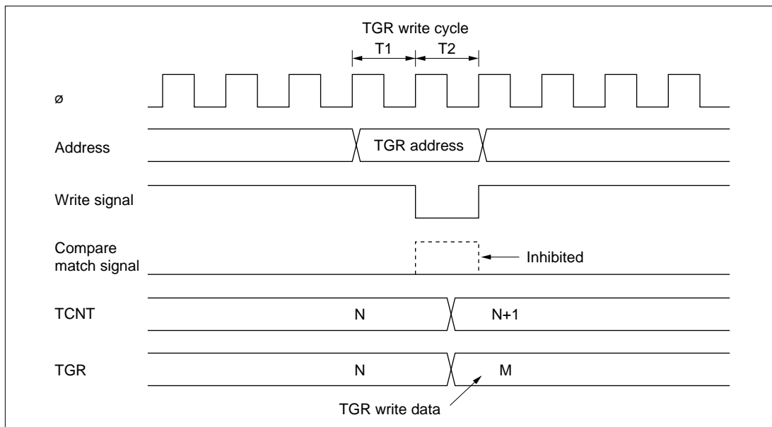
Figure 10-47 Contention between TGR Write and Compare Match
