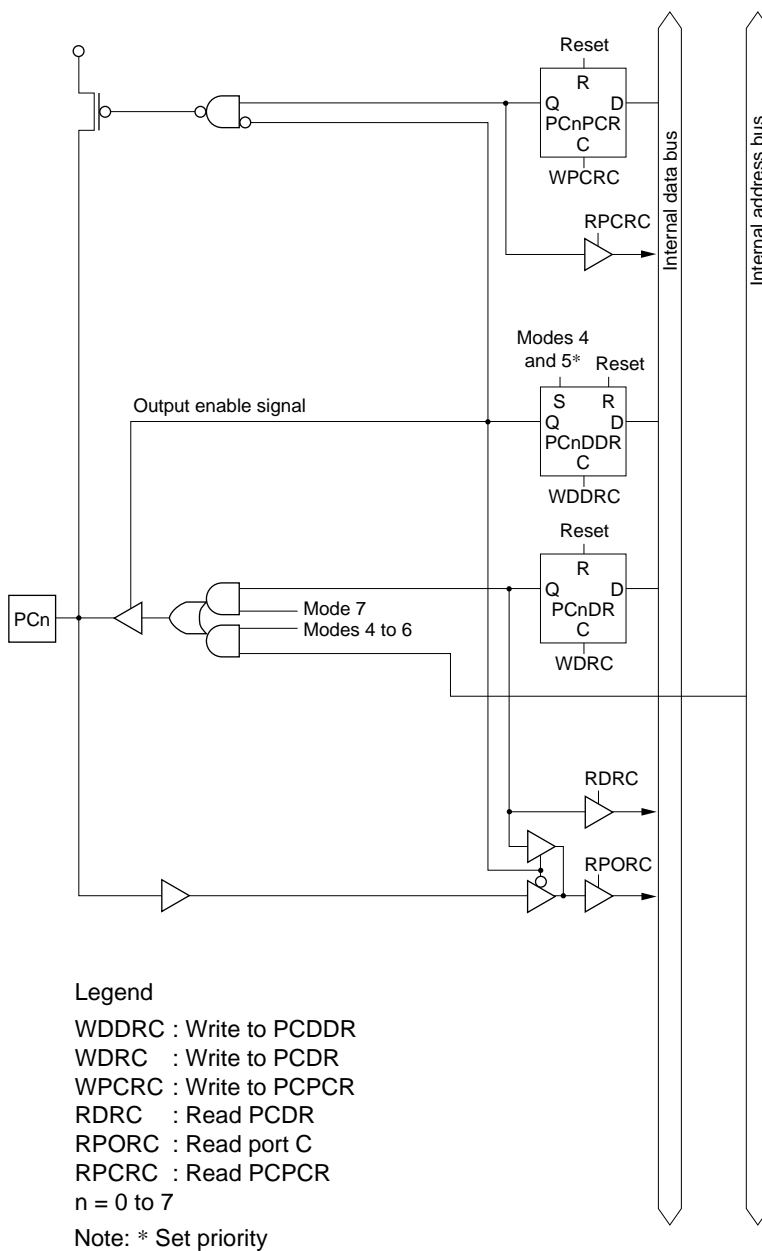
Figure C-22 Port C Block Diagram (Pins PC0 to PC7)
