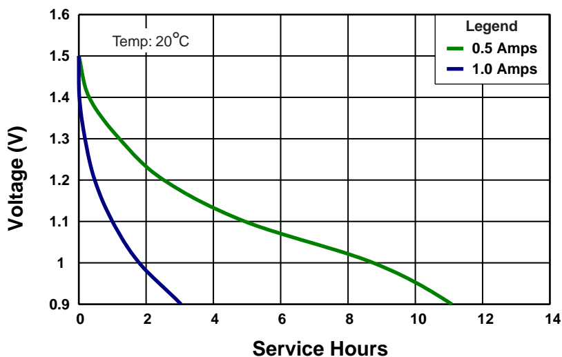
Typical Ultra C Discharge Characteristic
