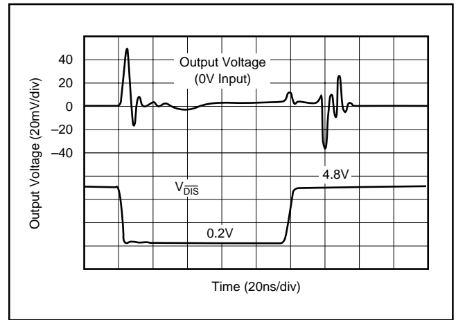
FIGURE 12. Disable/Enable Glitch.
