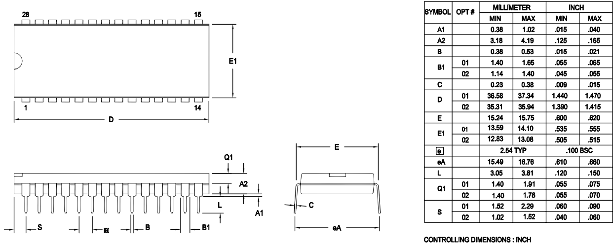
Figure 40 illustrates the 28-pin Plastic Dual Inline Package (PDIP) available for the Z8 Encore! XP ™ 8K Series devices.
