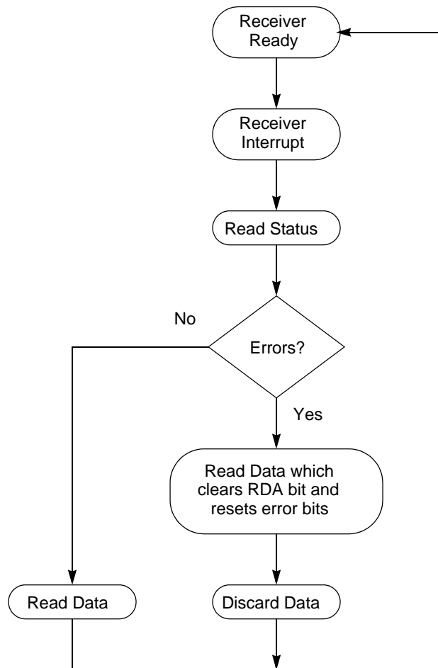
Figure 14. UART Receiver Interrupt Service Routine Flow
