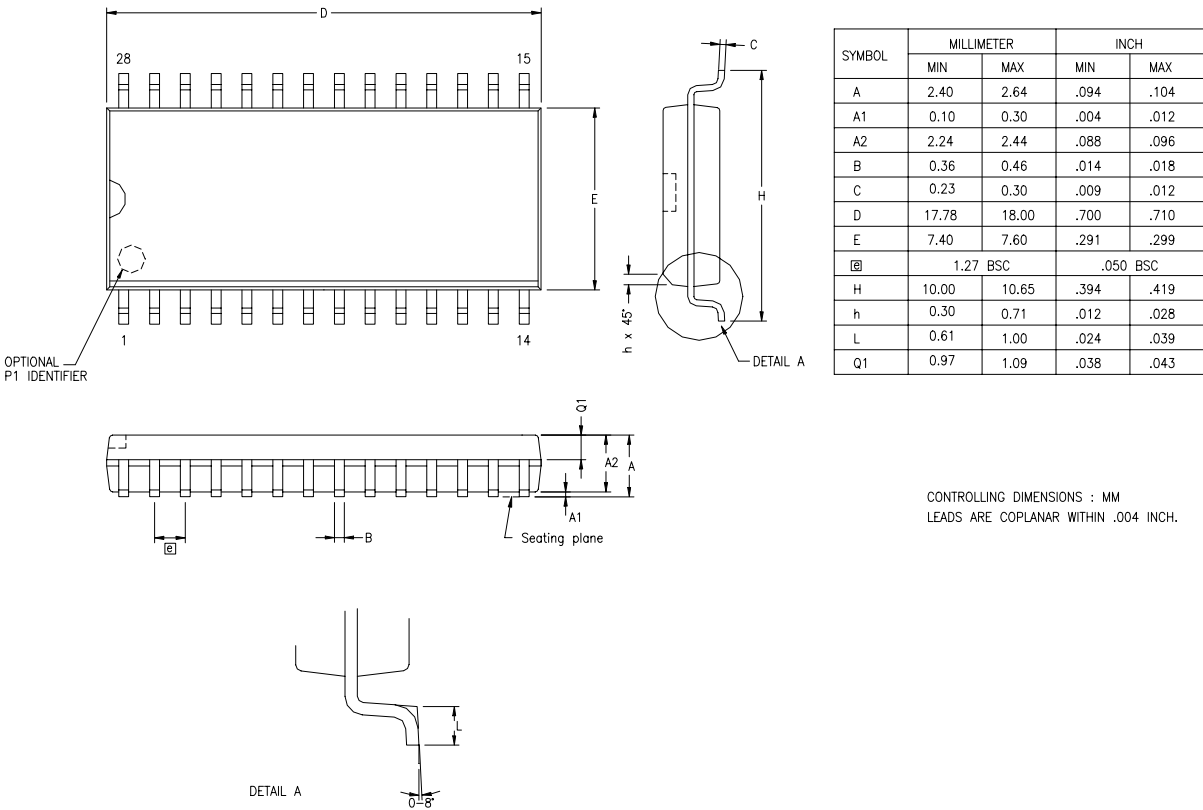
Figure 41 illustrates the 28-pin Small Outline Integrated Circuit package (SOIC) available in the Z8 Encore! XP ™ 8K Series devices.
