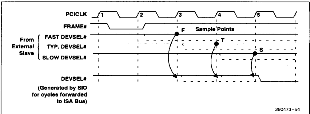
Figure 15. DEVSEL# Generation
