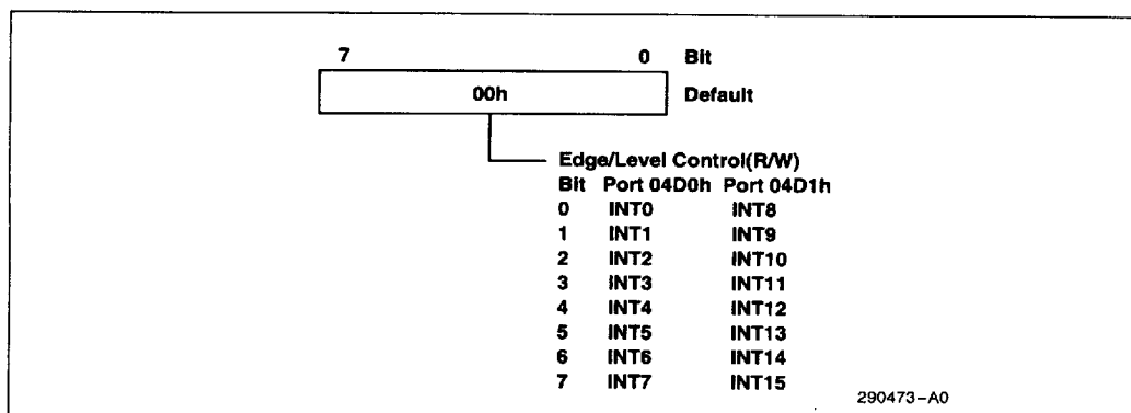
Figure 4. Edge/Level Select Register
