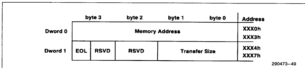
Figure 10. SGD Format
