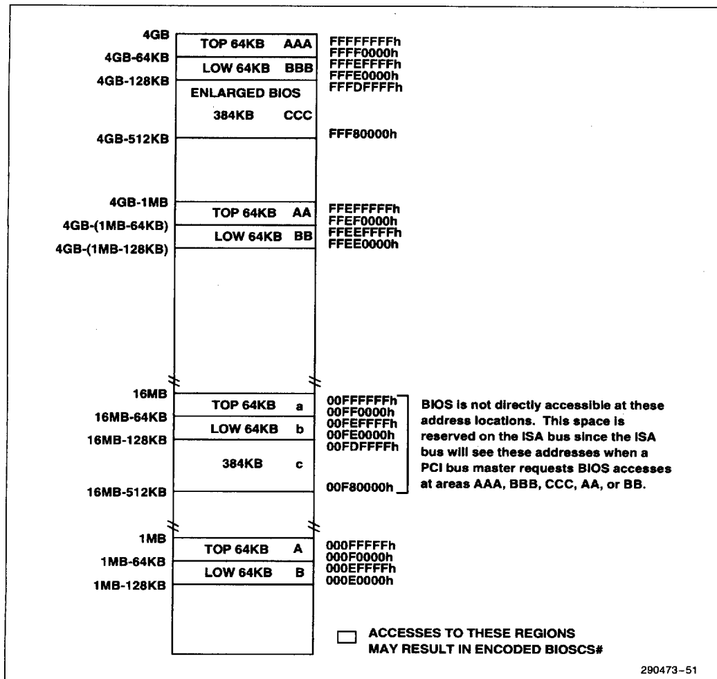
Figure 12. BIOS Space Decode Map
