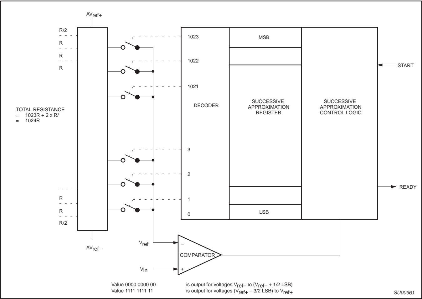
Figure 24. ADC Realization
