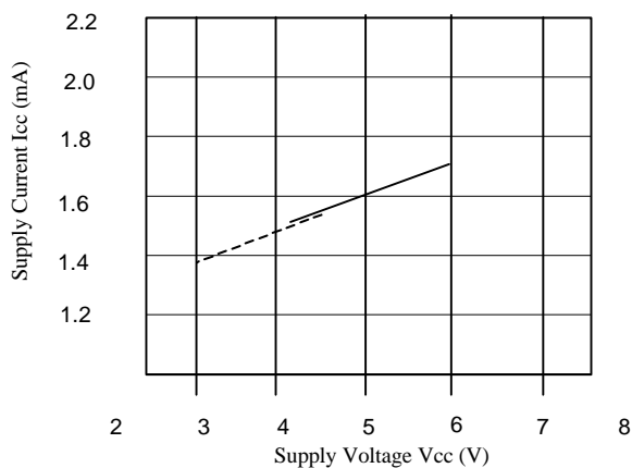
SUPPLY VOLTAGE vs. SUPPLY CURRENT
