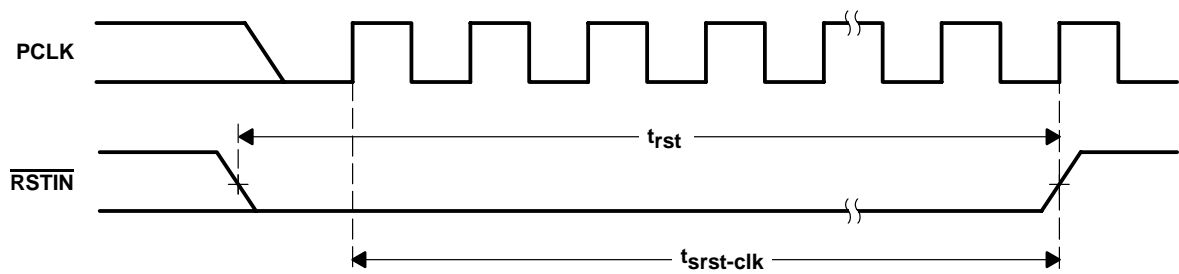
Figure 8-3. \overline{\text{RSTIN}} Timing Waveforms
