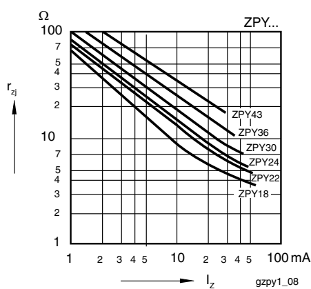
Fig. 5 - Dynamic Resistance vs. Zener Current
