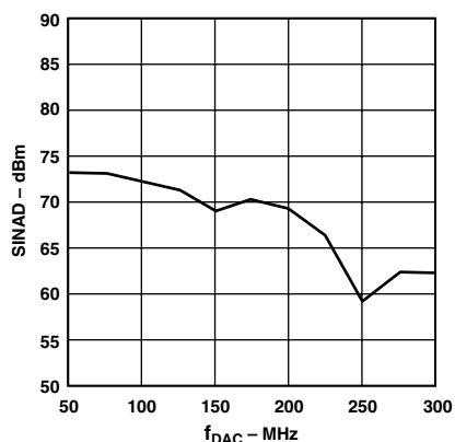
TPC 13. SINAD vs. f_{DAC} @ f_{OUT} = 10 \text{ MHz} , 0 \text{ dBFS}
