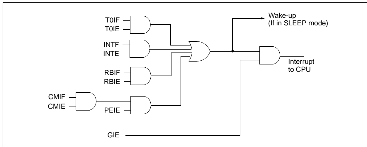
FIGURE 9-16: INTERRUPT LOGIC
