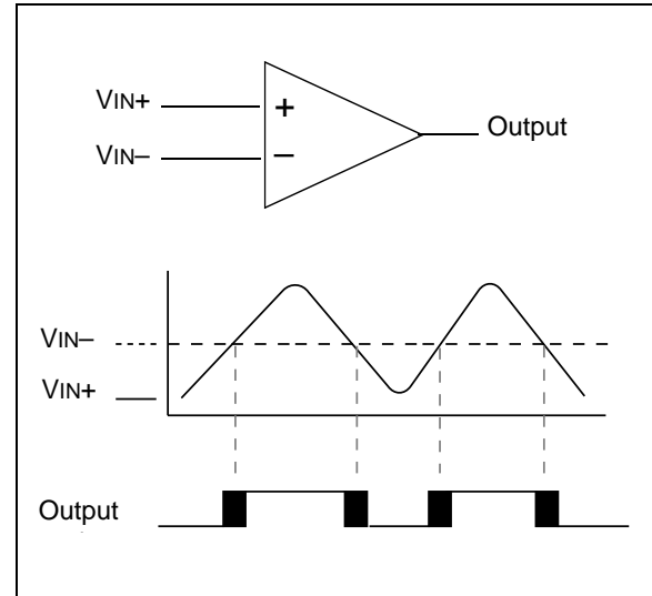
FIGURE 7-2: SINGLE COMPARATOR
