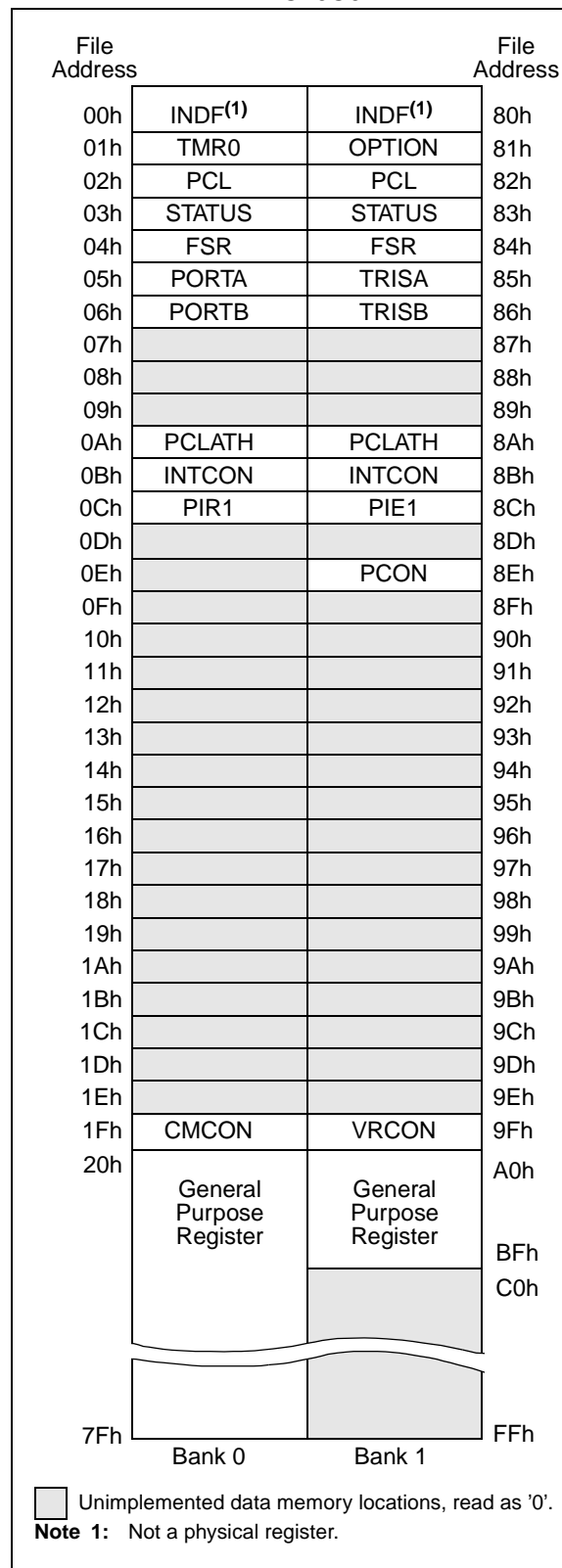
FIGURE 4-5: DATA MEMORY MAP FOR THE PIC16C622
