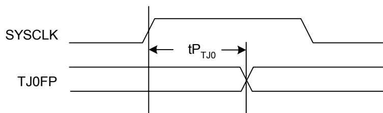
Figure 28 TSE Output Timing
