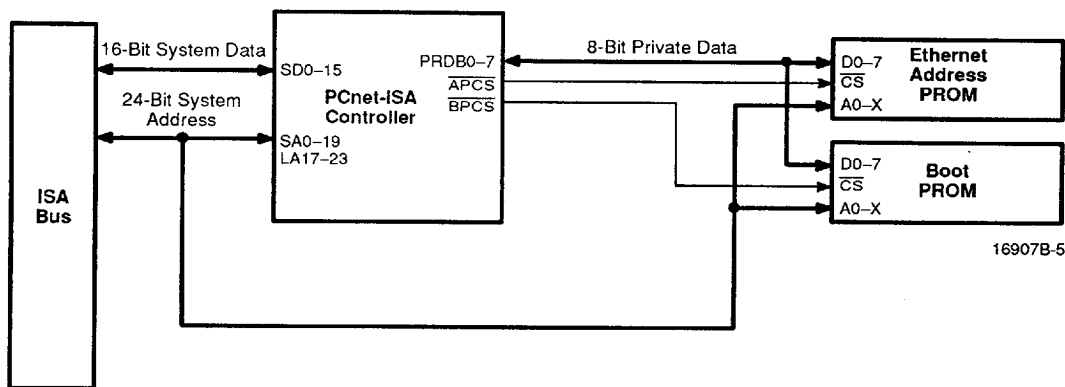
Bus Master Block Diagram
