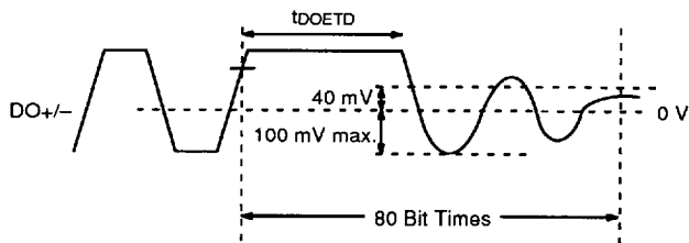
Port DO ETD Waveform
