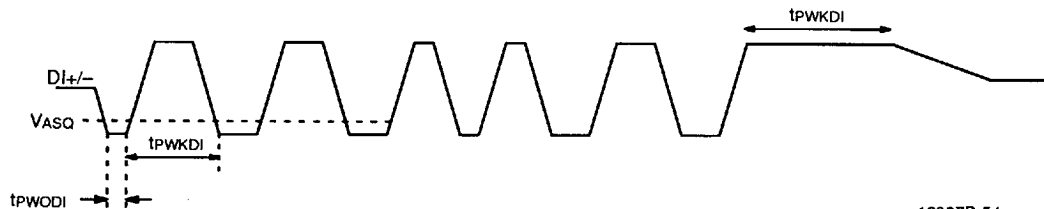
Receive Timing Diagram
