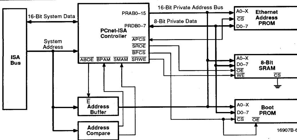
Shared Memory Block Diagram
