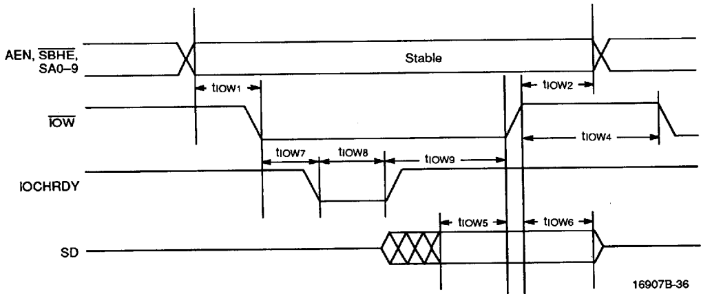
I/O Write with Wait States
