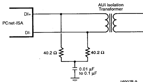
Differential Input Termination
