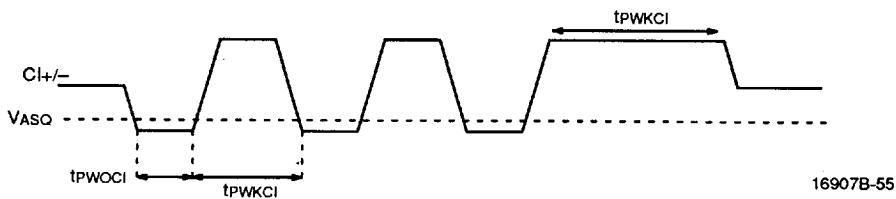
Collision Timing Diagram
