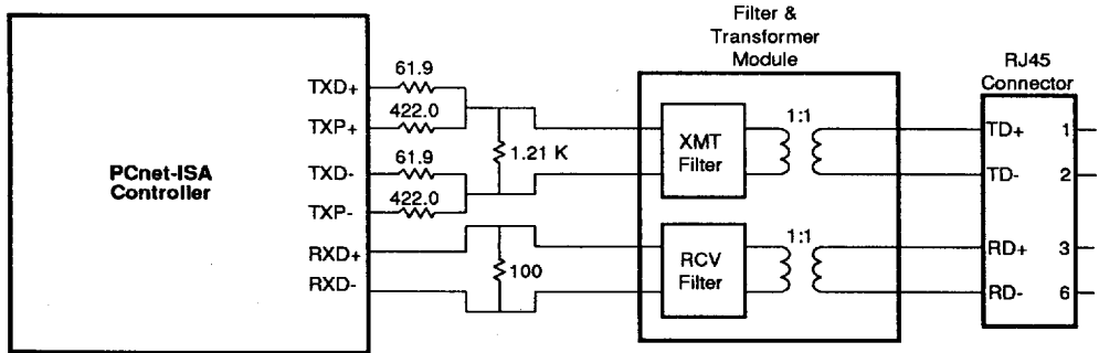
10BASE-T External Components and Hookup
