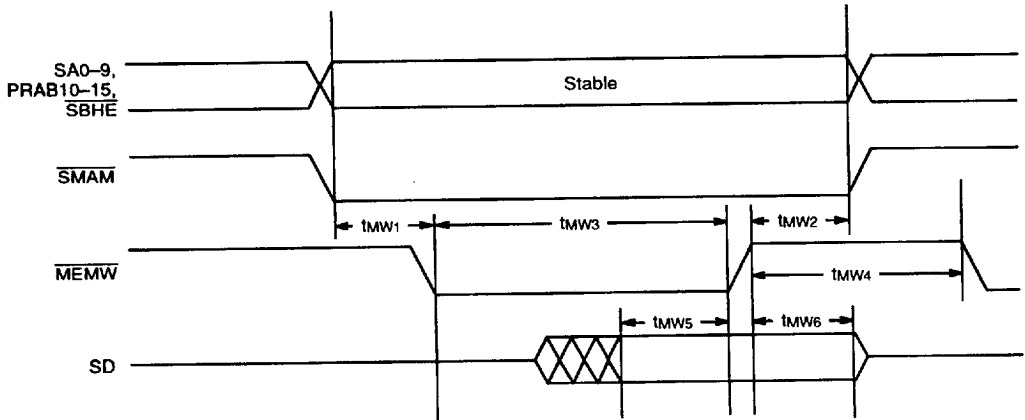
Memory Write without Wait States
