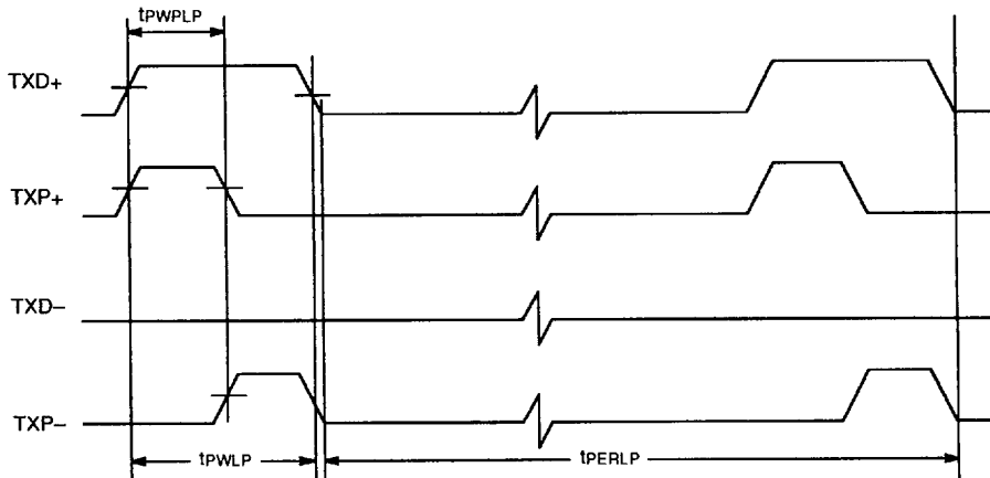
Idle Link Test Pulse
