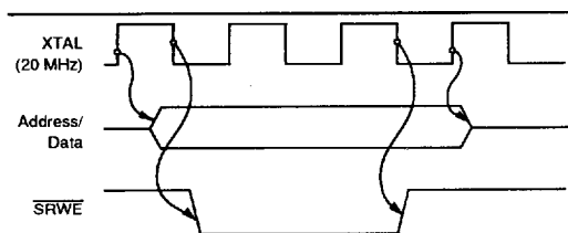
Static RAM Write Cycle
