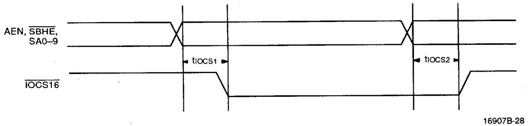
I/OCS16 Timings
