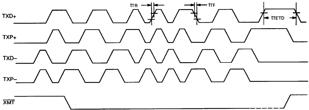
Transmit Timing
