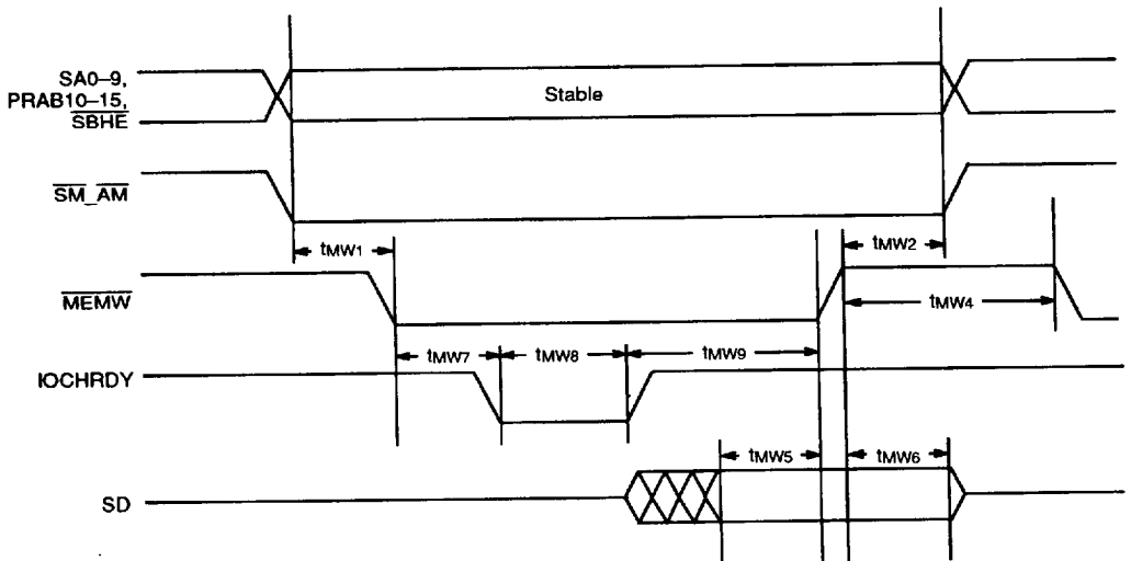
Memory Write with Wait States
