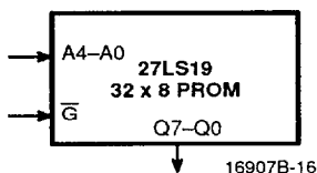
Address PROM Example
