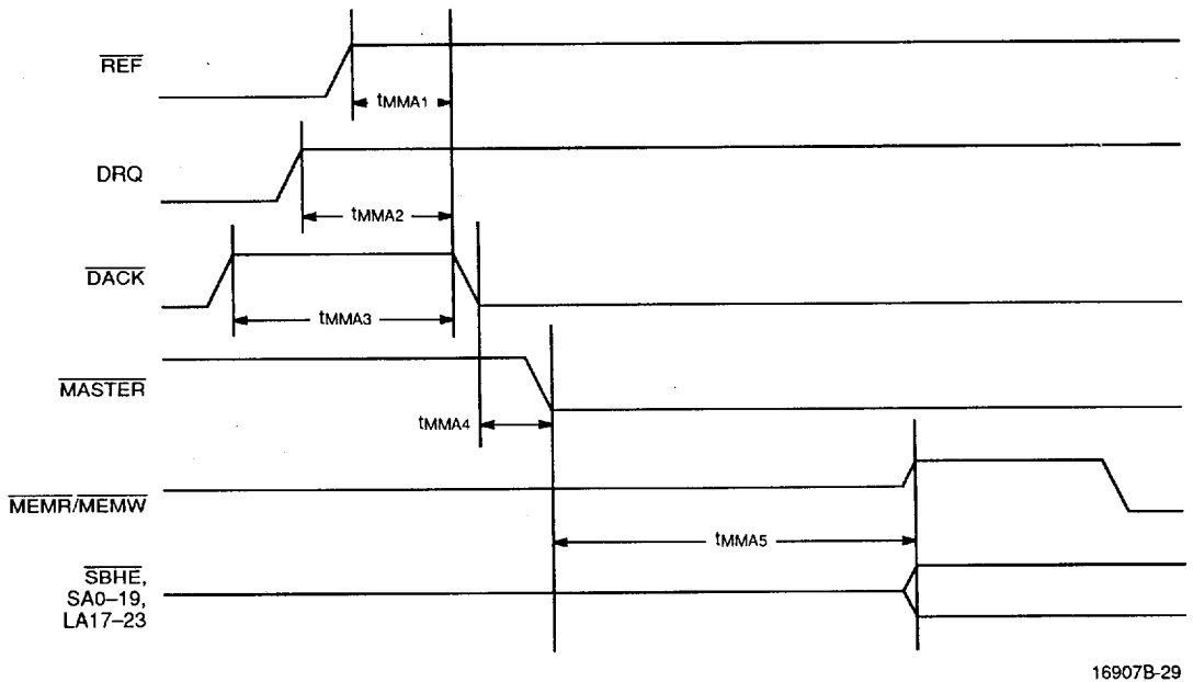
Bus Acquisition
