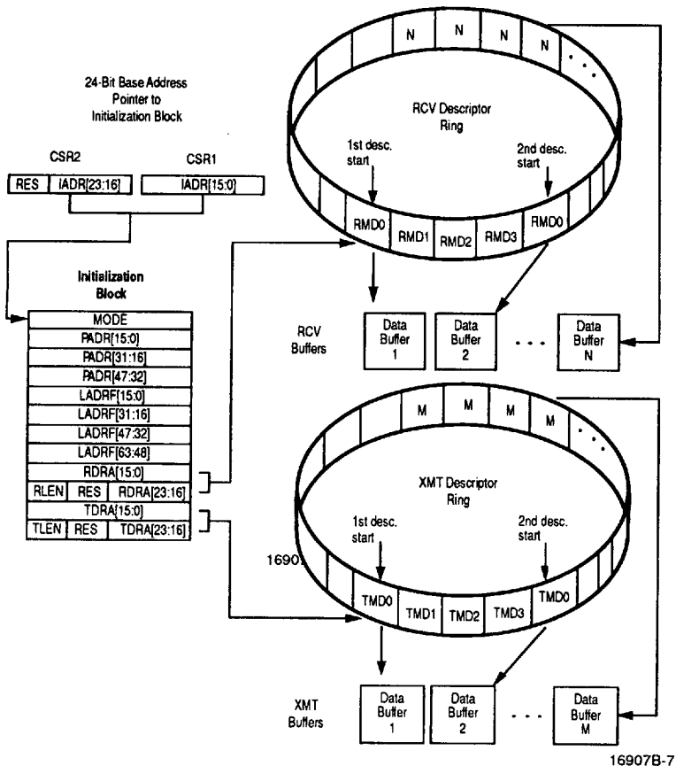
Initialization Block and Descriptor Rings
