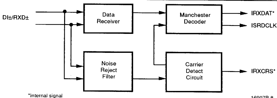
Receiver Block Diagram
