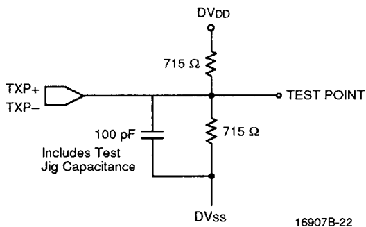
TXP Outputs Test Circuit
