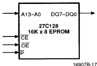
Boot PROM Example
