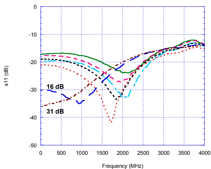
Figure 5. Input Return Loss at Major Attenuation Steps
