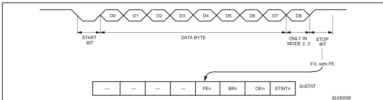
Figure 22. UART Framing Error Detection
