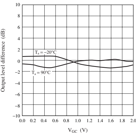
Output level — GC temperature characteristics ( 27^\circ\text{C} as reference)
