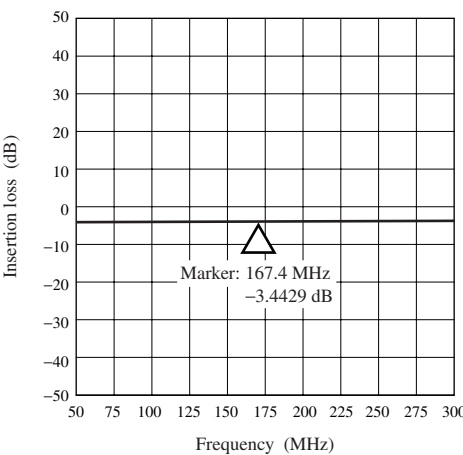
Balance transformer insertion loss (S21)
