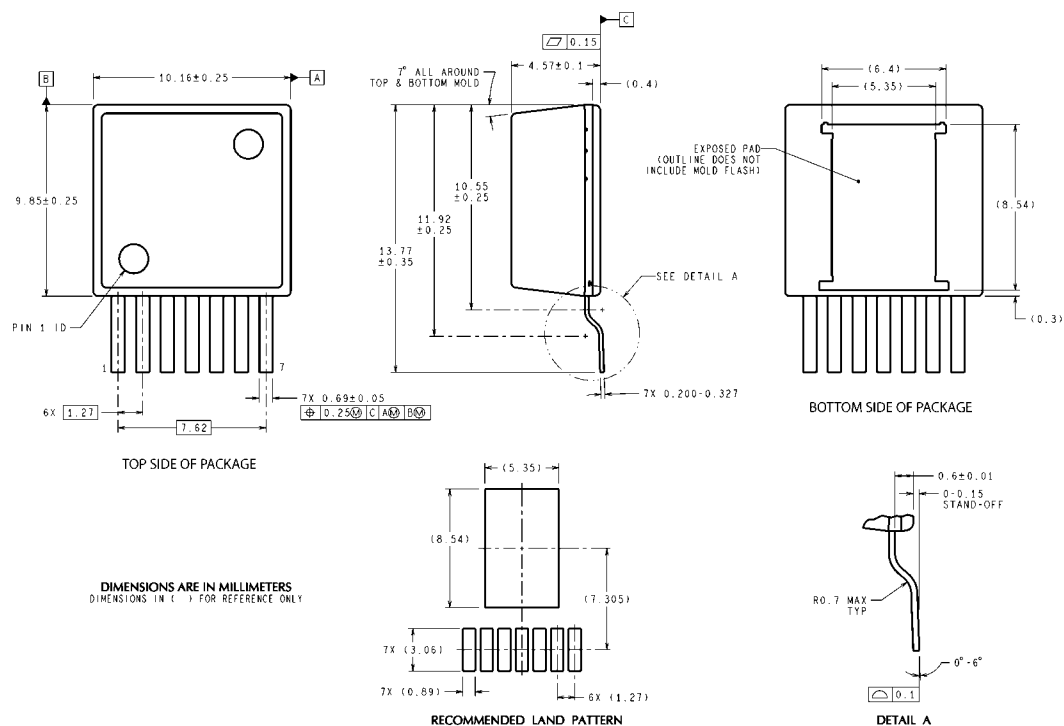
7-Lead TZA Package NS Package Number TZA07A
