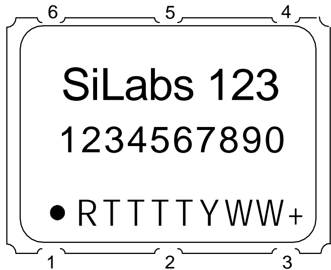
Figure 3. Mark Specification
