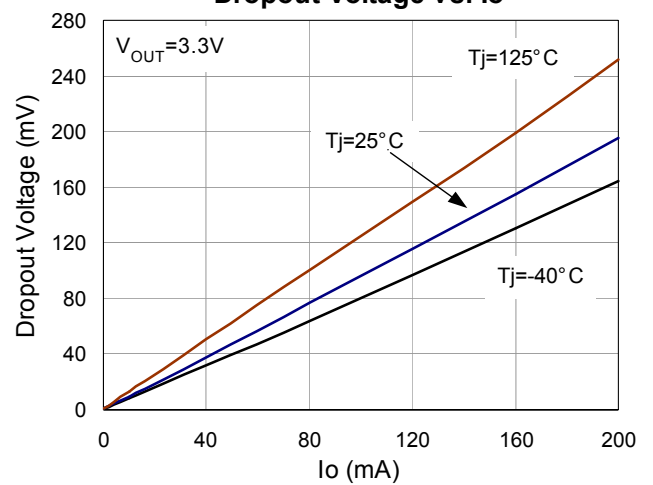
Dropout Voltage vs. I_O
