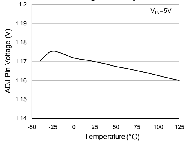
ADJ Pin Voltage vs. Temperature
