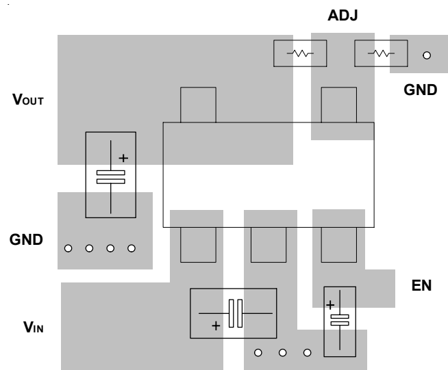
SOT-25 Board Layout
