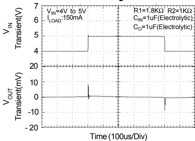
Line Regulation
