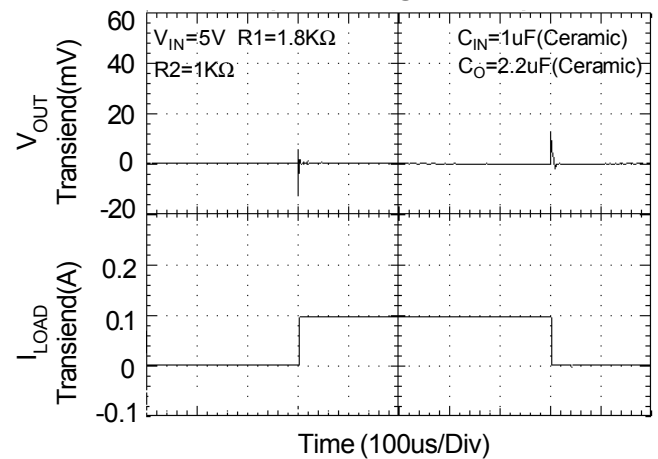
Load Regulation
