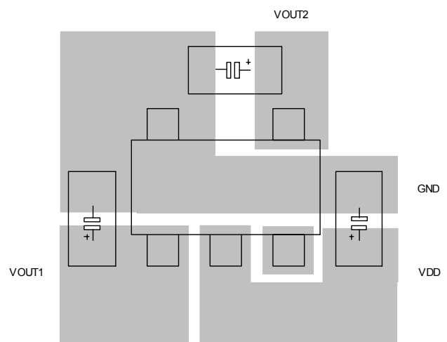
SOT-25 Board Layout
