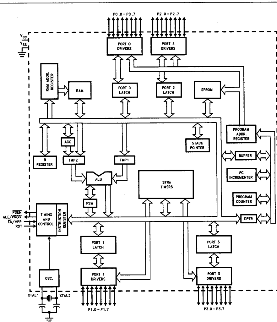
Figure 1. 8XC5X Block Diagram
