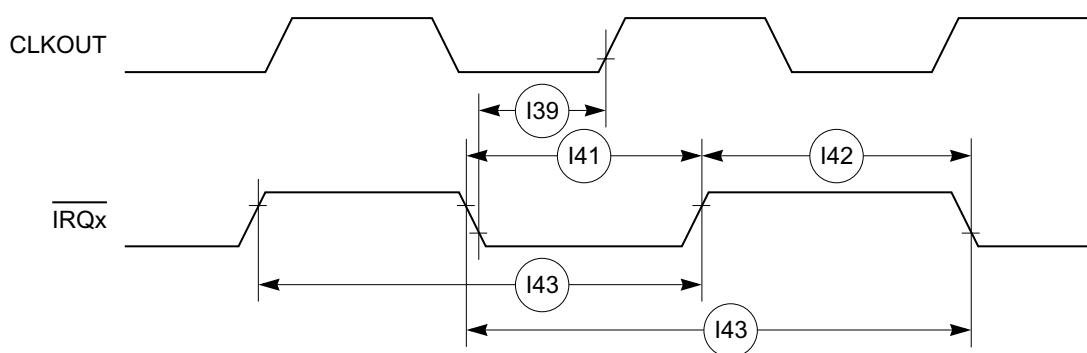
Figure 6-23. Interrupt Detection Timing for External Edge Sensitive Lines
