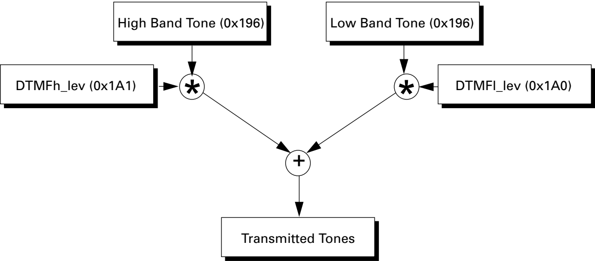
Figure 9. Transmitting Tones
