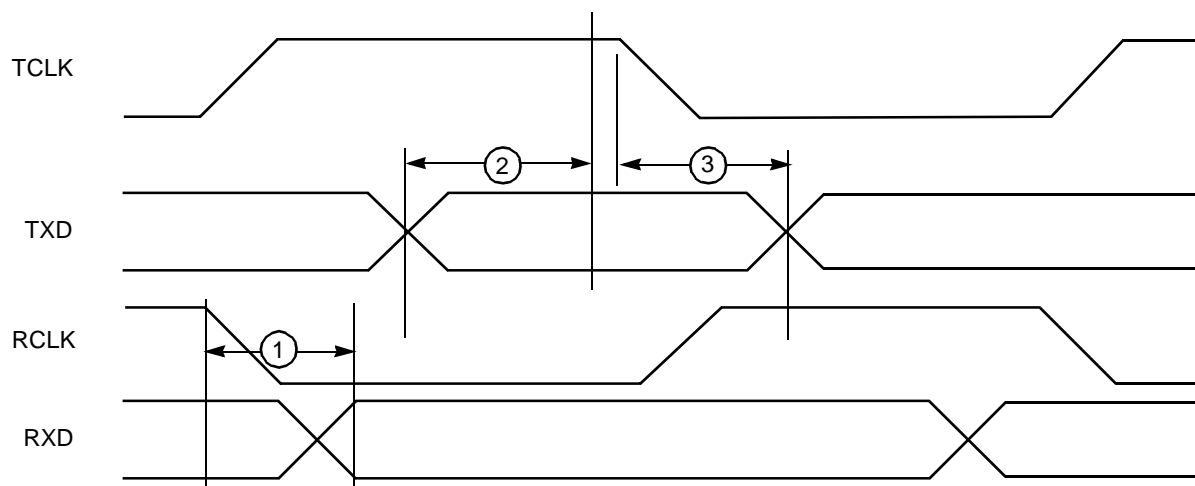
Figure 10. Serial Port Timing Diagram
