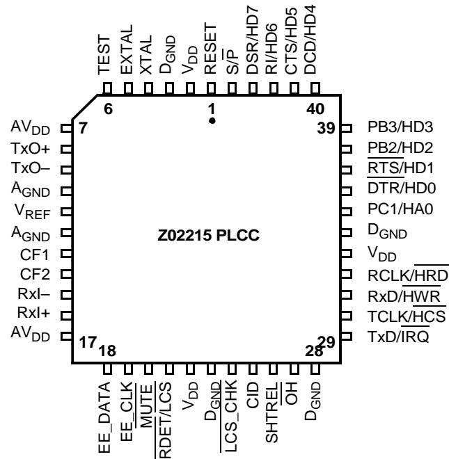
Figure 2. Z02215 44-Lead PLCC Pin Identification (for Prototype Only)
