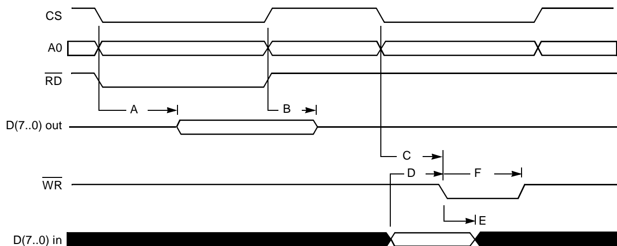
Figure 11. Parallel Port Timing
