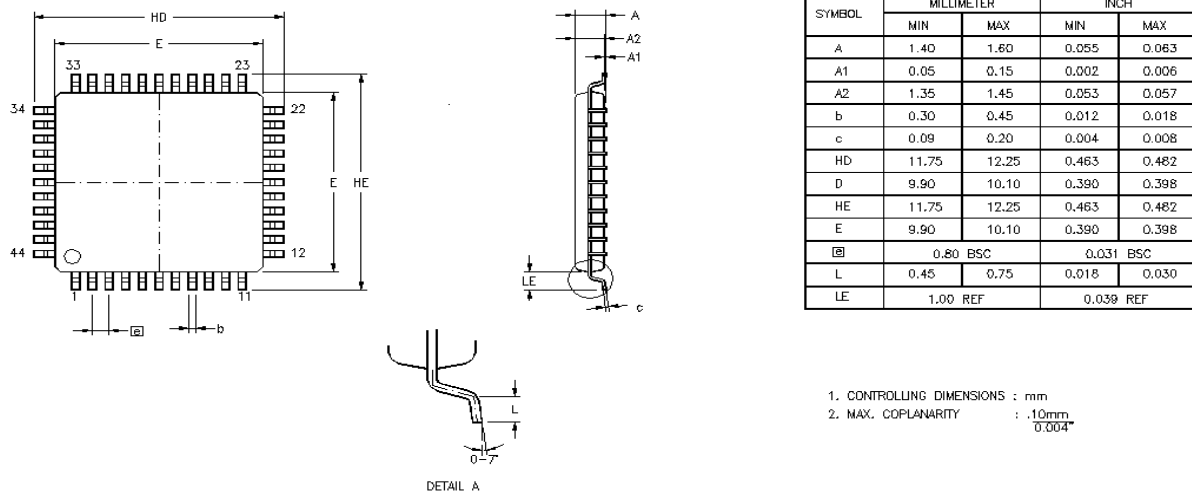
Figure 13. 44-Lead VQFP Package Diagram
