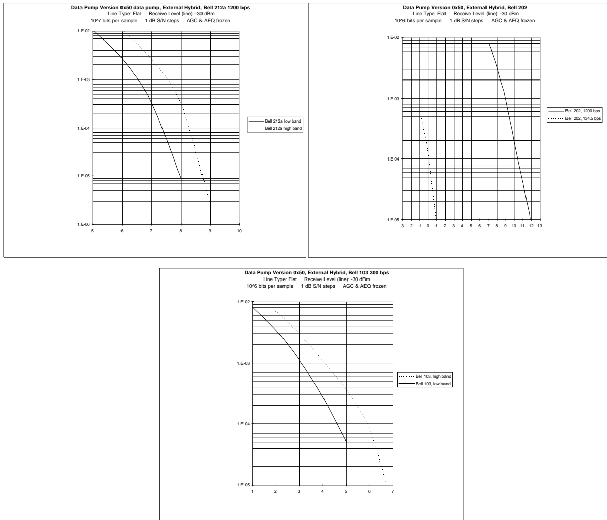
Figure 6. Typical Performance Data (continued)
