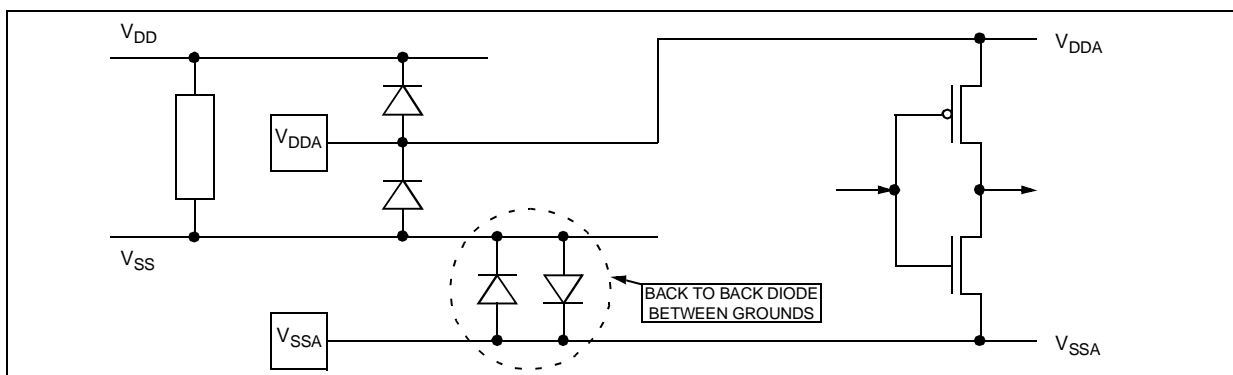
Figure 68. Multisupply Configuration
