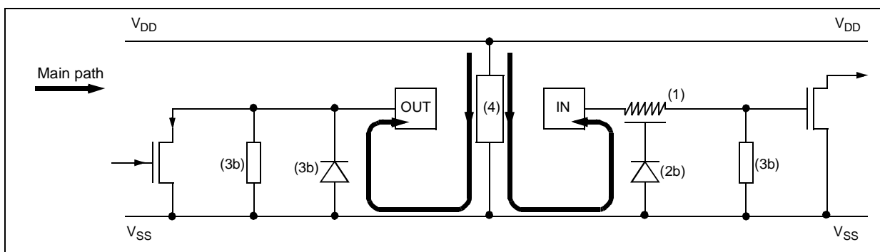
Figure 68. Multisupply Configuration
