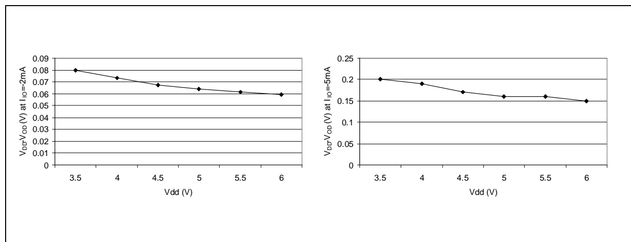
Figure 79. Typical V_{DD}-V_{OH} vs. V_{DD} (high sink port)
