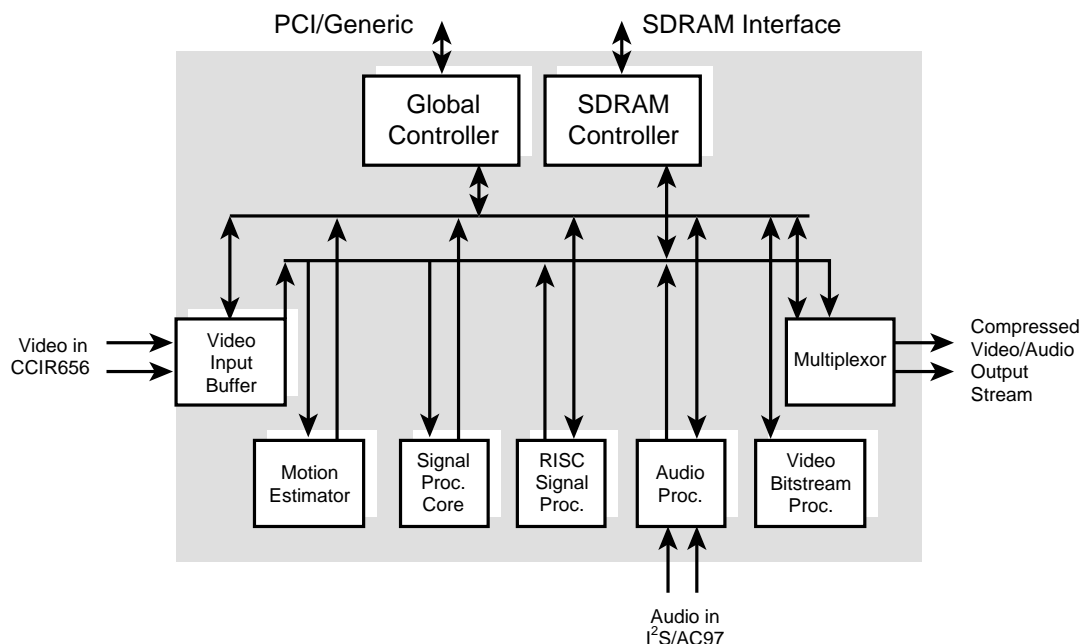
BCM7041 Block Diagram
