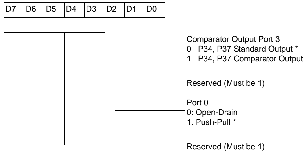
PCON (FH) 00H
