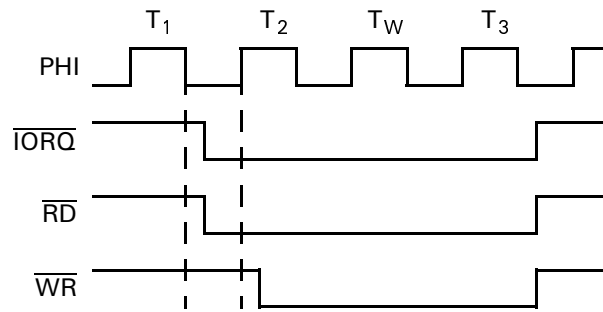
Figure 11. I/O Read and Write Cycles with \overline{\text{IOC}} = 1
