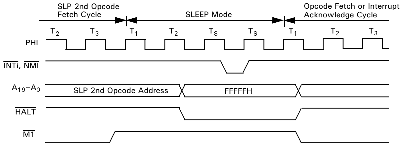
Figure 14. SLEEP Timing
