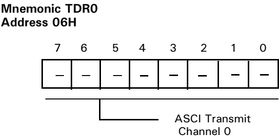
Figure 36. ASCI Register
