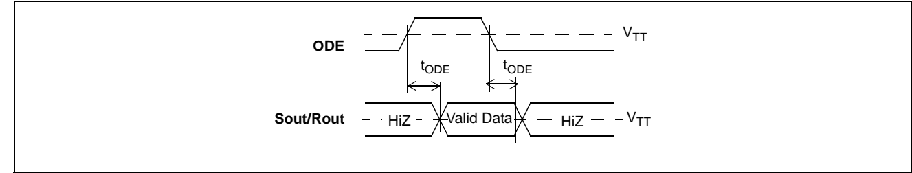
Figure 13 - Output Driver Enable (ODE)
