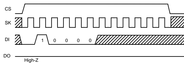
Fig.14 Write disable cycle timing (WDS)
