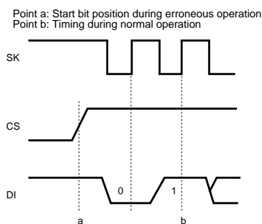
Fig.16 Erroneous operation timing
