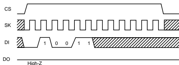
Fig.11 Write enable cycle timing
