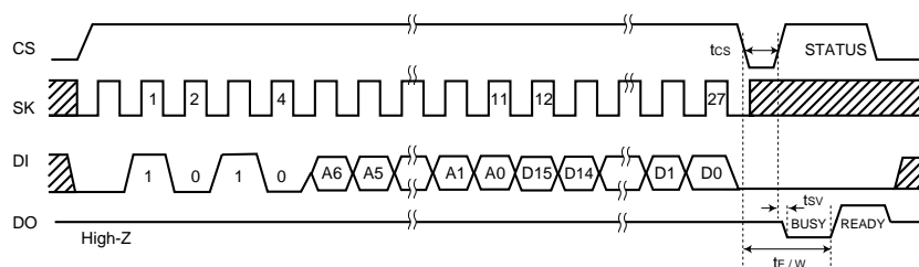
Fig.12 Write cycle timing (WRITE)
