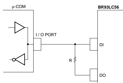
Fig.19 Common connections for the DI and DO control line
