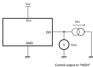
Fig.4 "HIGH" output voltage circuit
