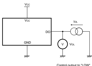
Fig.3 "LOW" output voltage circuit
