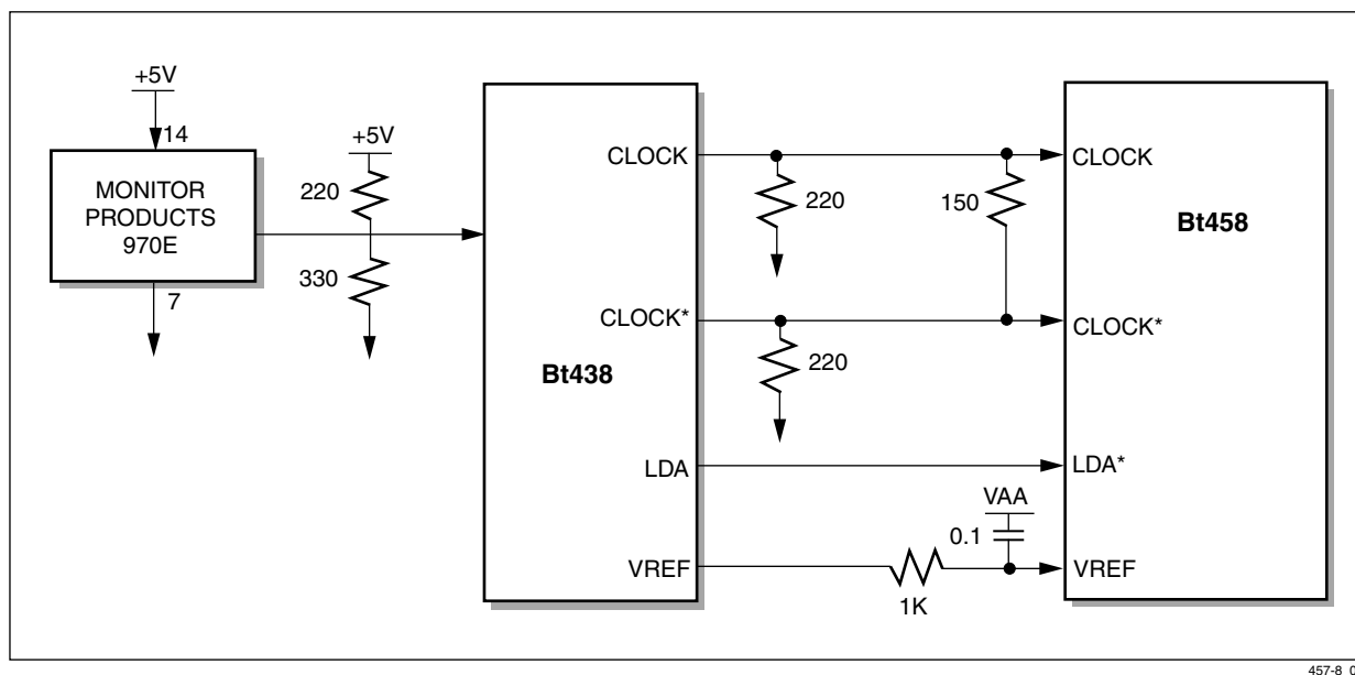
Figure 4-1. Generating the Bt458 Clock Signals
