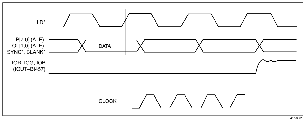
Figure 1-3. Video Input/Output Timing
