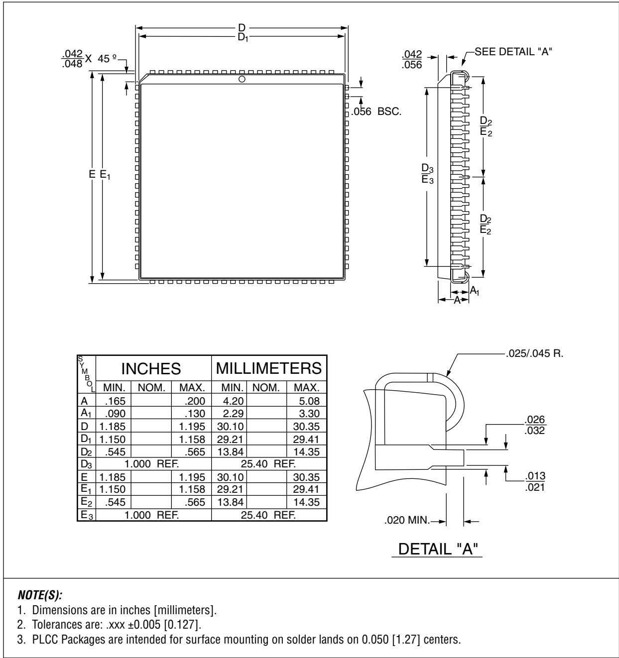
Figure 5-3. 84-Pin Plastic J-Lead (PLCC)
