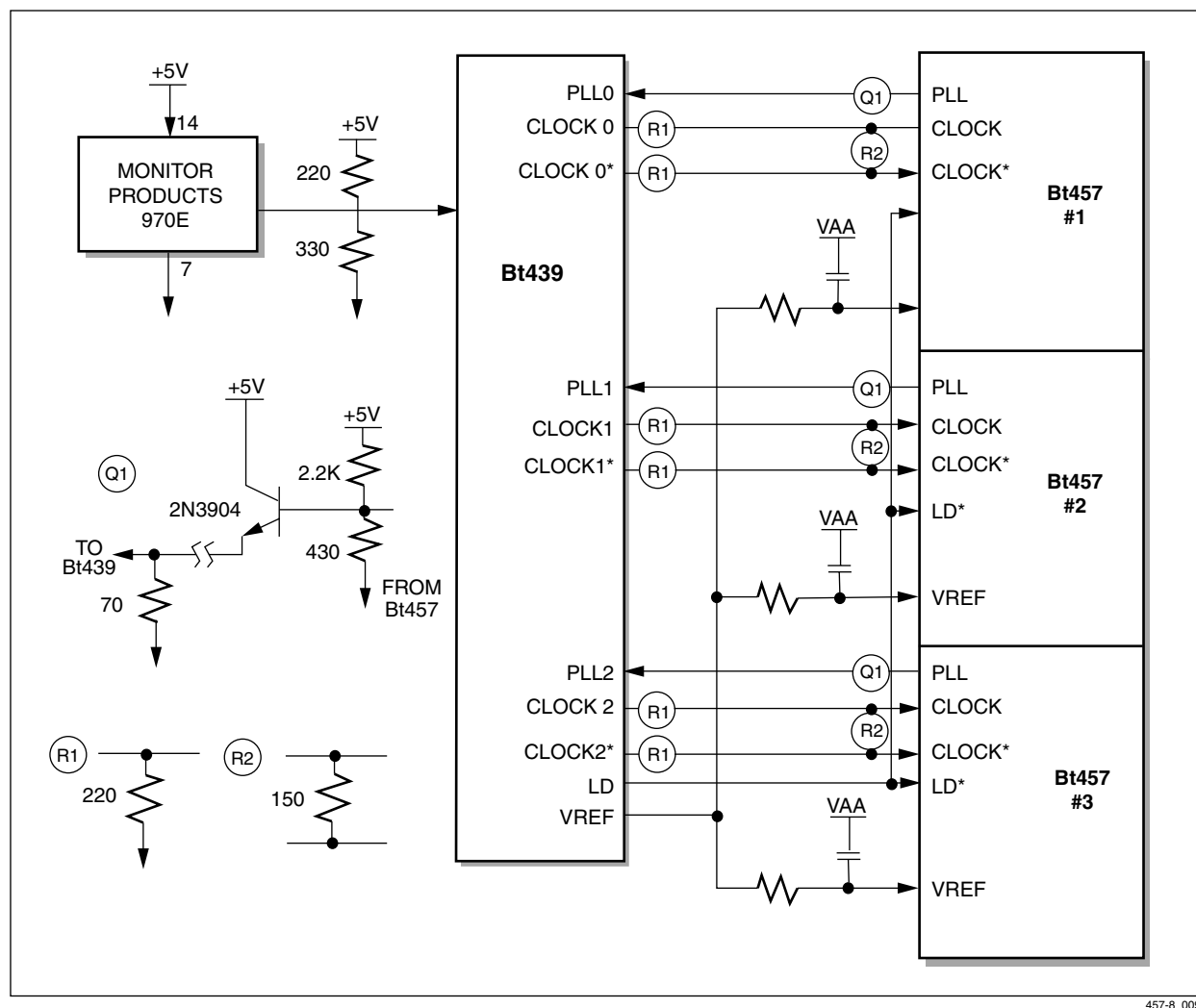
Figure 4-3. Generating the Bt457 Clock Signals (Color Application)
