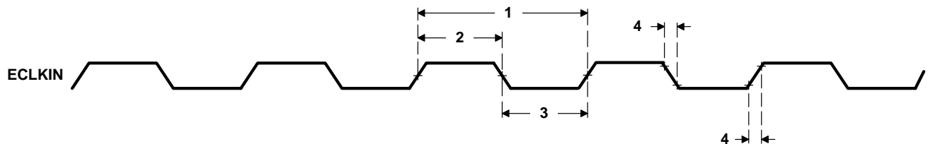
Figure 16. ECLKIN Timing for EMIFA and EMIFB
