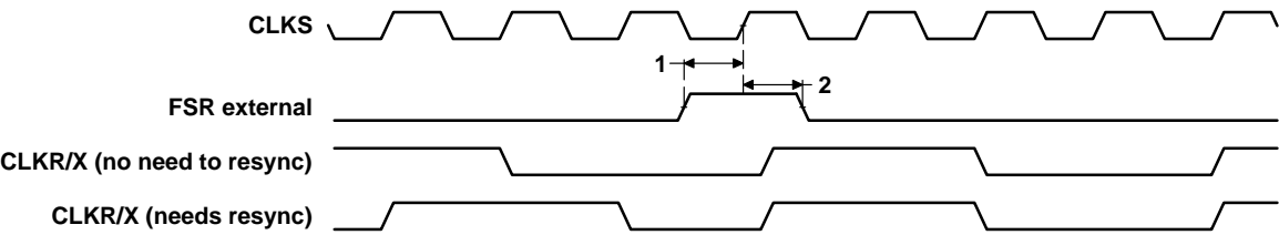
Figure 49. FSR Timing When GSYNC = 1
