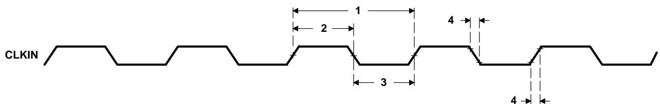
Figure 13. CLKIN Timing
