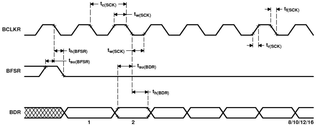
Figure 35. Buffered Serial Port Receive Timing
