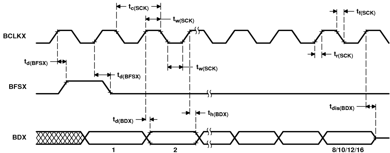
Figure 37. Buffered Serial Port Transmit Timing of Internal Clocks and Internal Frames
