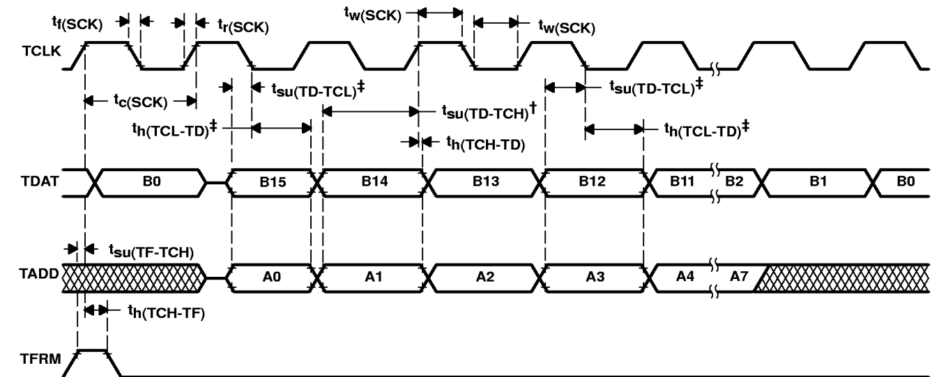
Figure 38. Serial-Port Receive Timing in TDM Mode
