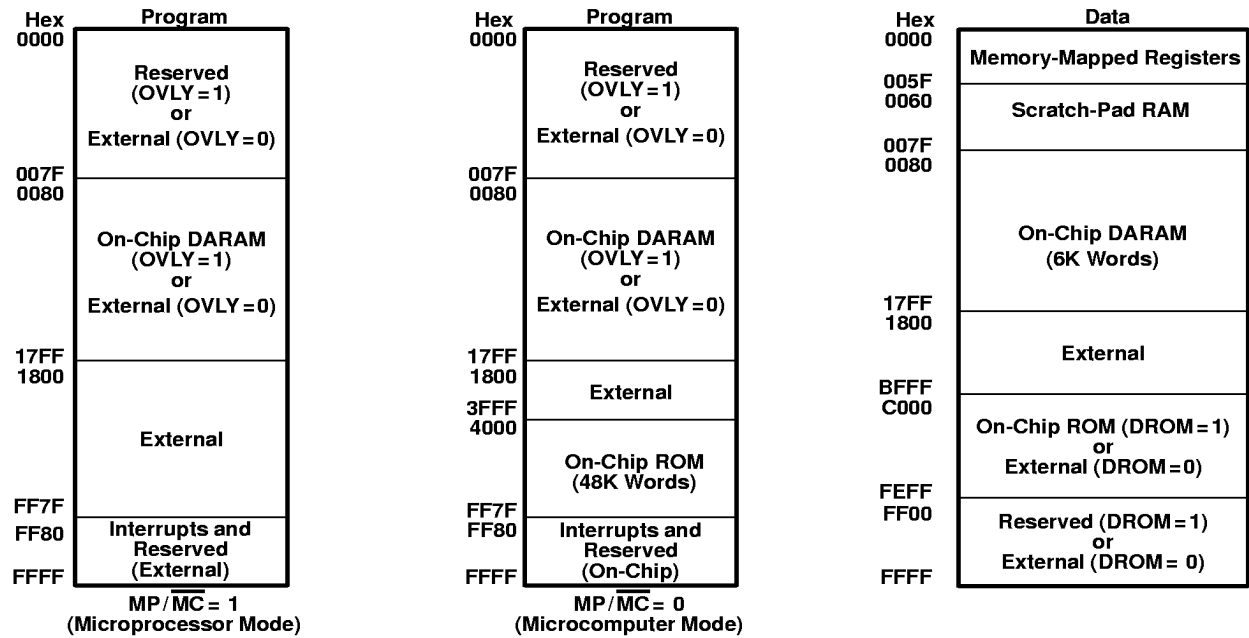
Figure 3. Memory Map ('545 and '546 only)
