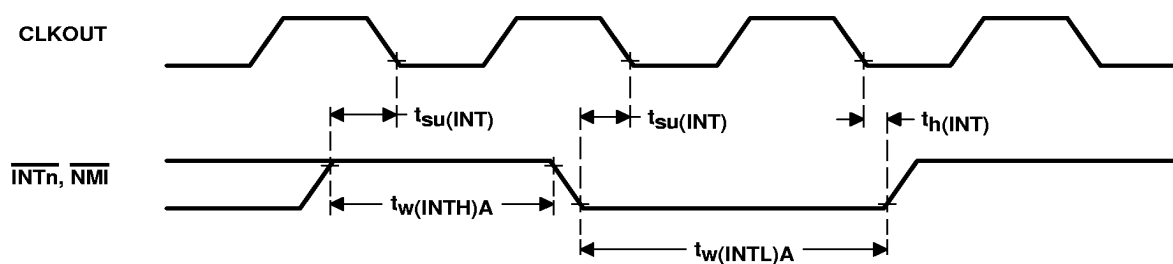
Figure 27. Interrupt Timing
