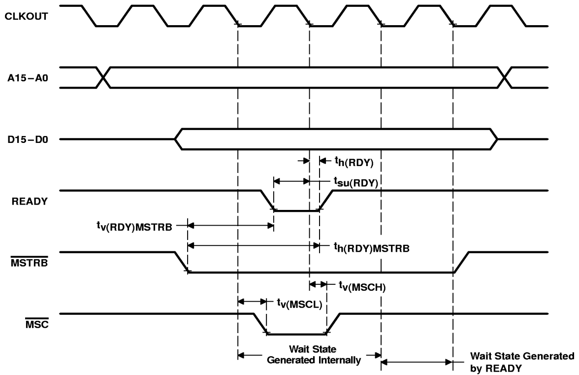
Figure 22. Memory Write With Externally Generated Wait States
