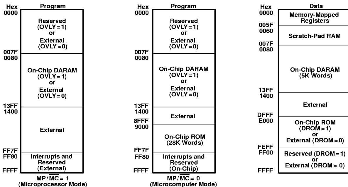
Figure 1. Memory Map ('541 only)
