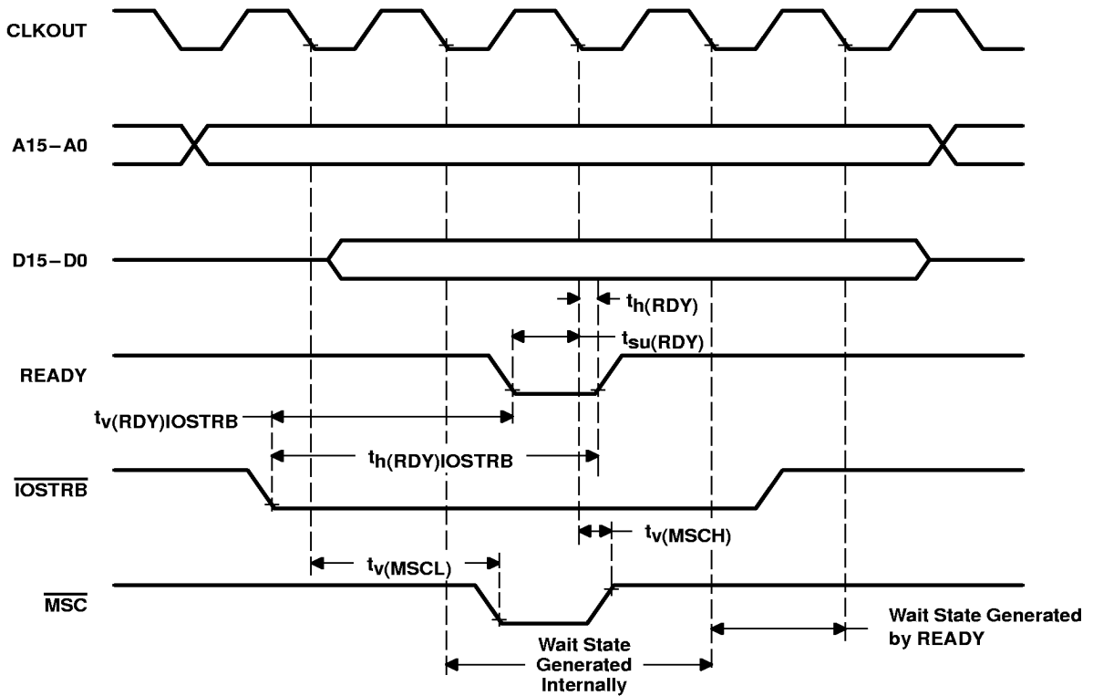
Figure 24. I/O Write With Externally Generated Wait States
