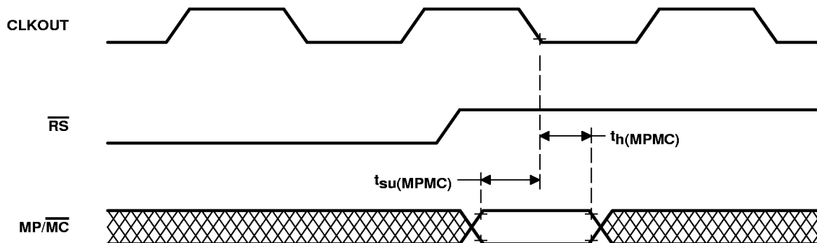
Figure 28. \text{MP}/\overline{\text{MC}} Timing
