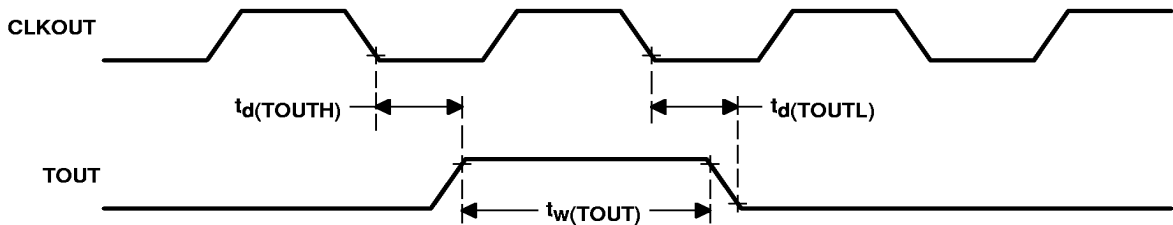
Figure 31. TOUT Timing
