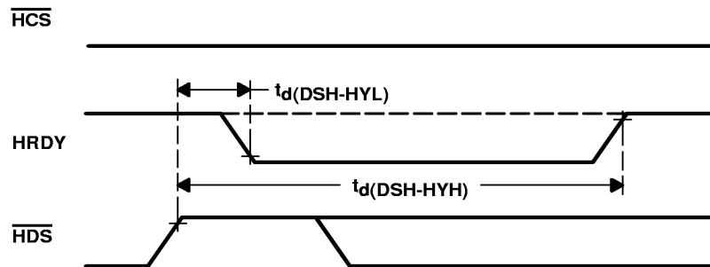
Figure 43. \text{HRDY} Signal When \overline{\text{HCS}} is Always Low
