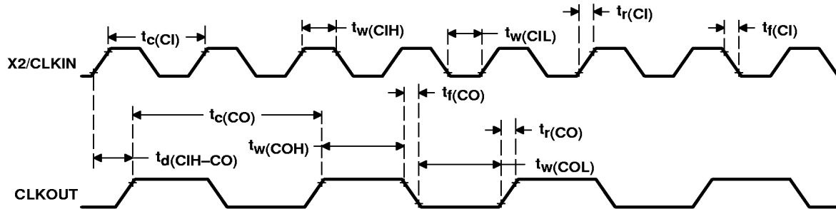
Figure 14. External Divide-by-Two Clock Timing
