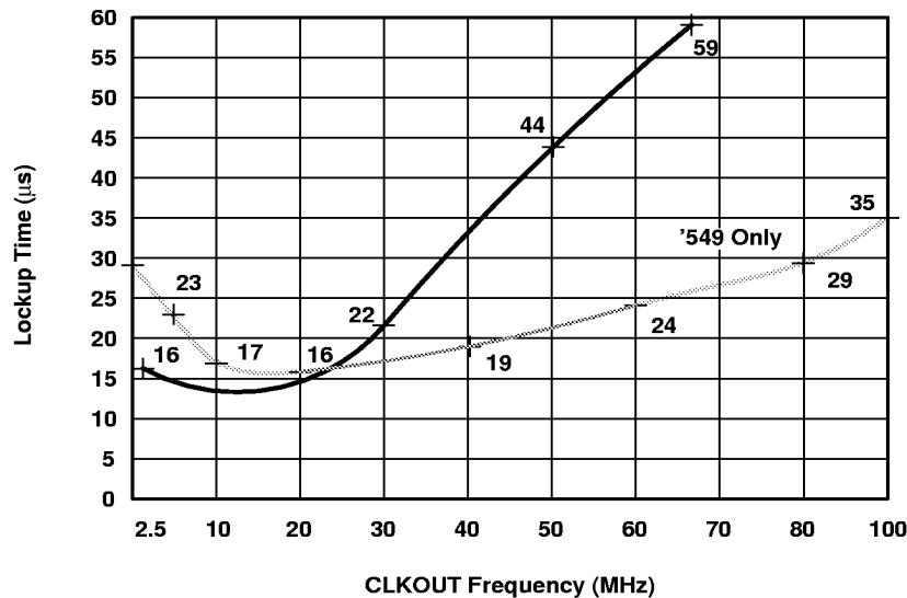
Figure 8. PLL Lockup Time Versus CLKOUT Frequency
