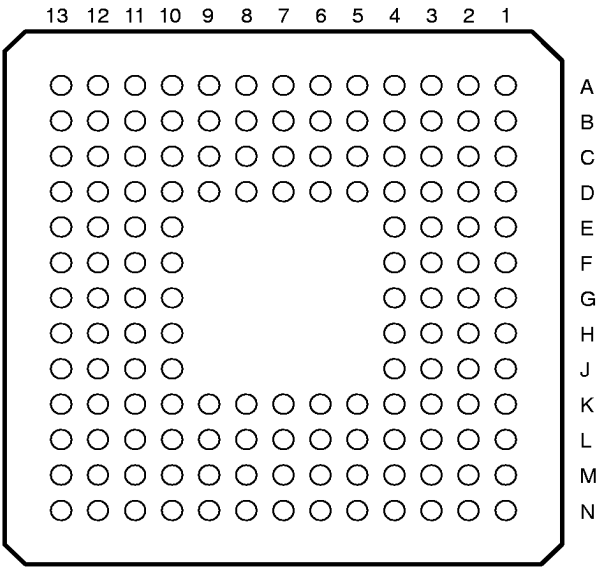
TMS320LC548, TMS320LC549, TMS320VC549 GGU PACKAGE (BOTTOM VIEW)
