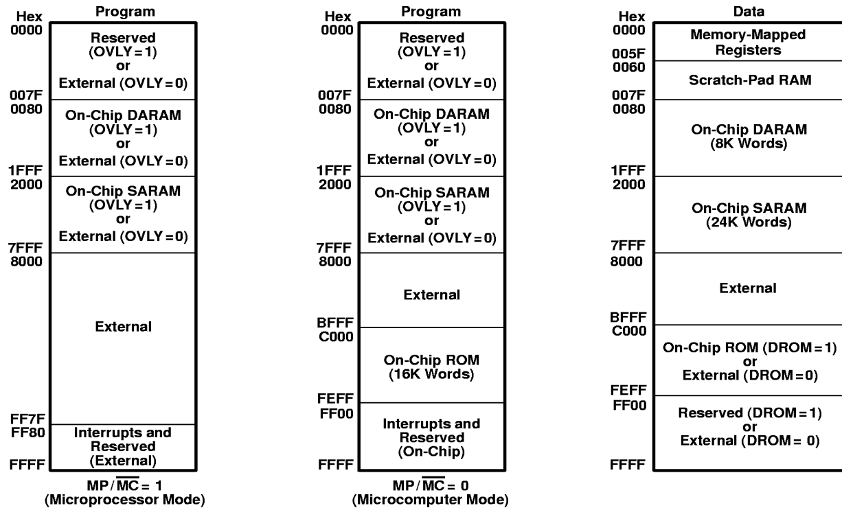
Figure 5. Memory Map ('549 only)
