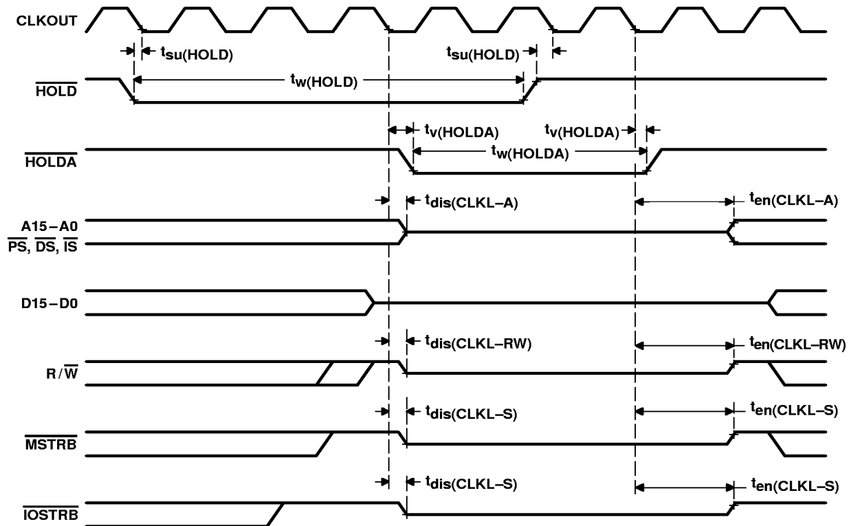
Figure 25. HOLD and HOLDA Timing (HM = 1)
