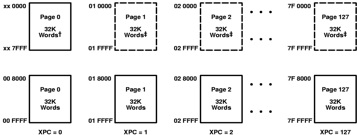
Figure 5. Memory Map ('549 only)
