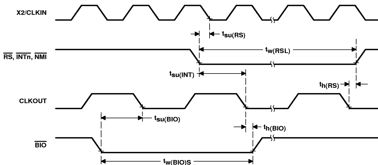
Figure 26. Reset and \overline{\text{BIO}} Timings
