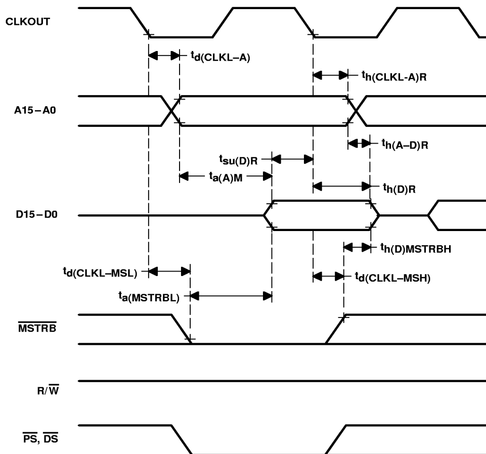
Figure 16. Memory Read ( \overline{\text{MSTRB}} = 0 )
