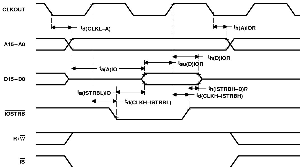
Figure 18. Parallel I/O Port Read ( \overline{\text{IOSTRB}} = 0 )
