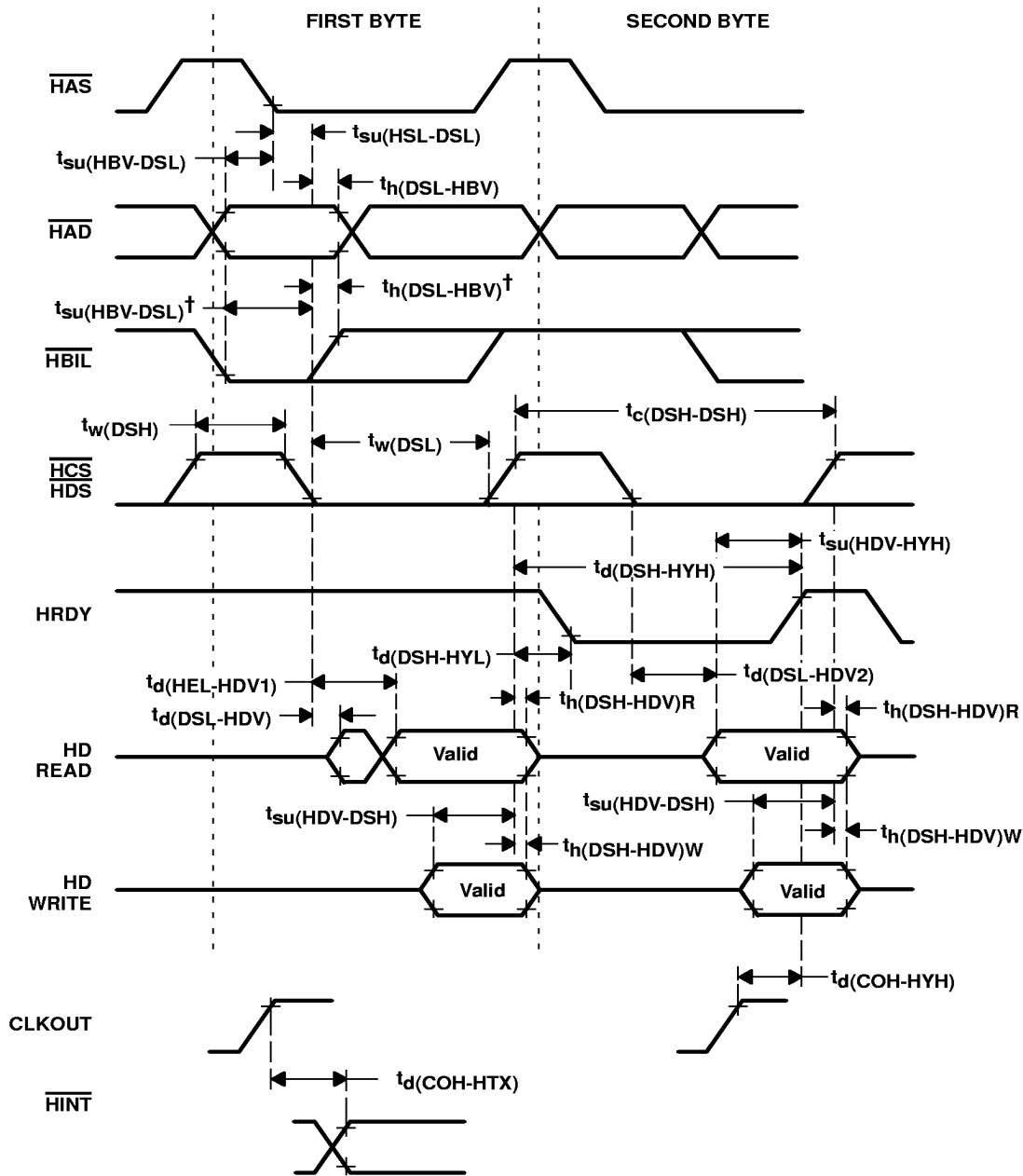
Figure 42. Read/Write Access Timing With HRDY
