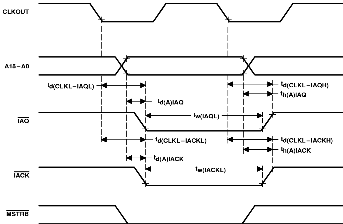
Figure 29. Instruction Acquisition ( \overline{\text{IAQ}} ) and Interrupt Acknowledge ( \overline{\text{IACK}} ) Timing
