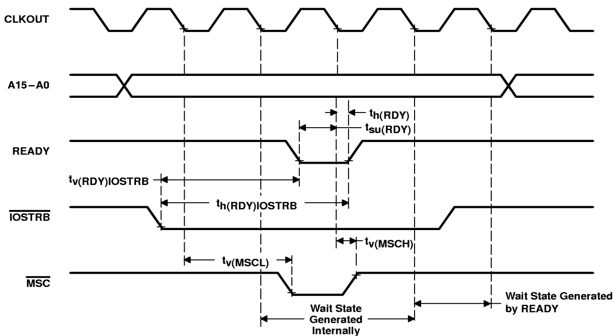
Figure 23. I/O Read With Externally Generated Wait States
