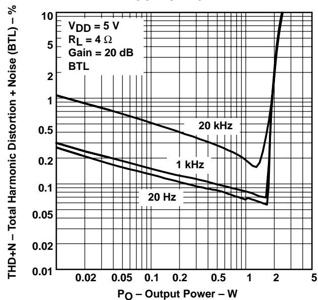
TOTAL HARMONIC DISTORTION + NOISE (BTL) vs OUTPUT POWER
