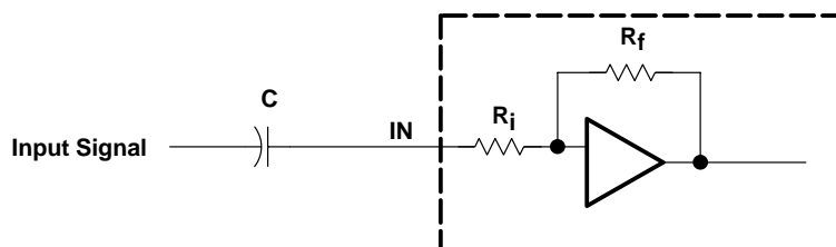
Figure 34. Resistor on Input for Cut-Off Frequency
