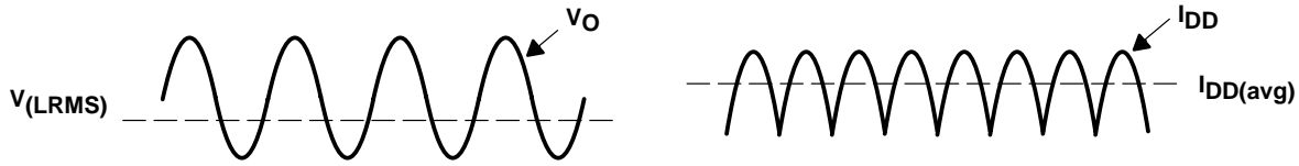
Figure 37. Voltage and Current Waveforms for BTL Amplifiers
