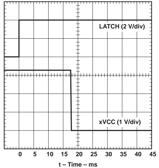
Figure 4. xVCC Propagation Delay and Fall Time With 1-μF Load, 3.3-V Switch
