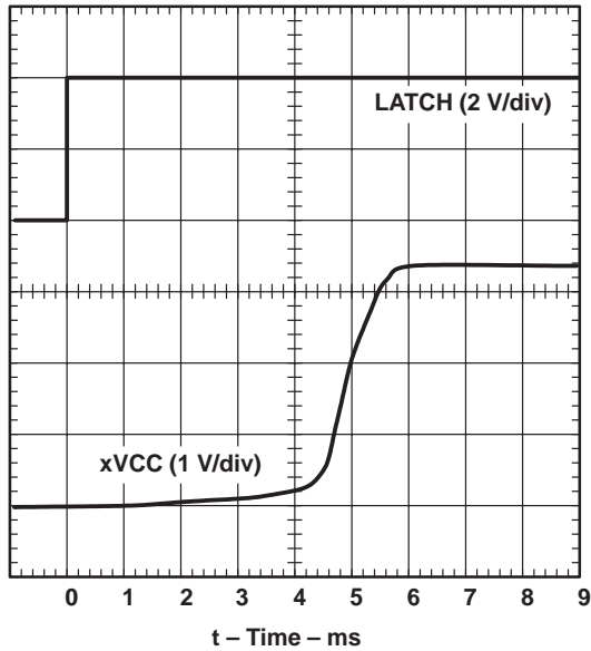
Figure 3. xVCC Propagation Delay and Rise Time With 1-μF Load, 3.3-V Switch
