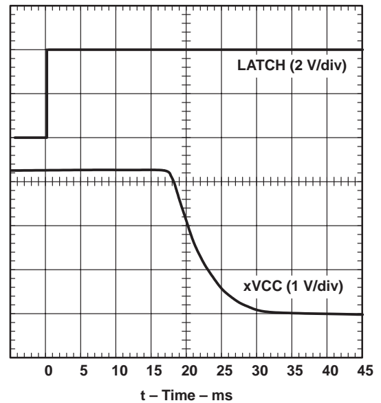
Figure 6. xVCC Propagation Delay and Fall Time With 100-μF Load, 3.3-V Switch
