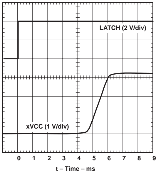
Figure 5. xVCC Propagation Delay and Rise Time With 100-μF Load, 3.3-V Switch
