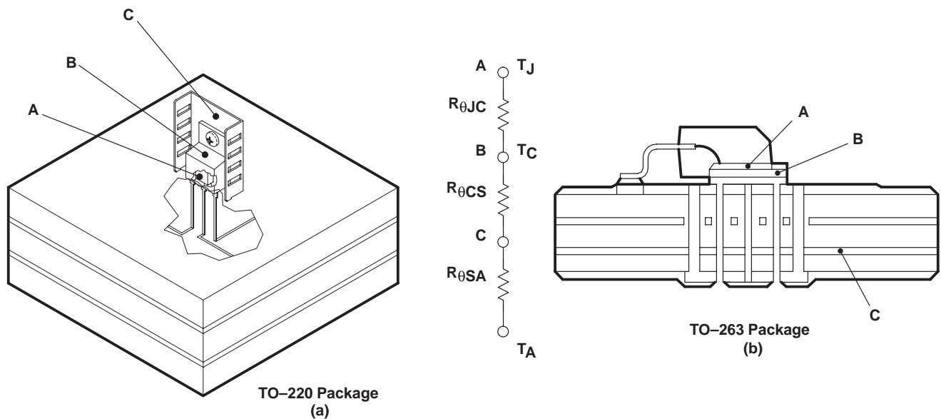
Figure 21. Thermal Resistances
