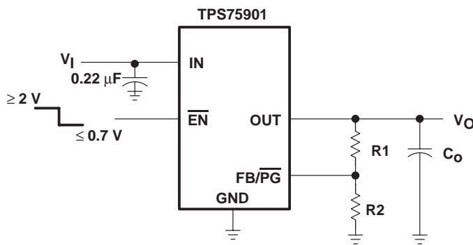
Figure 28. TPS75901 Adjustable LDO Regulator Programming
