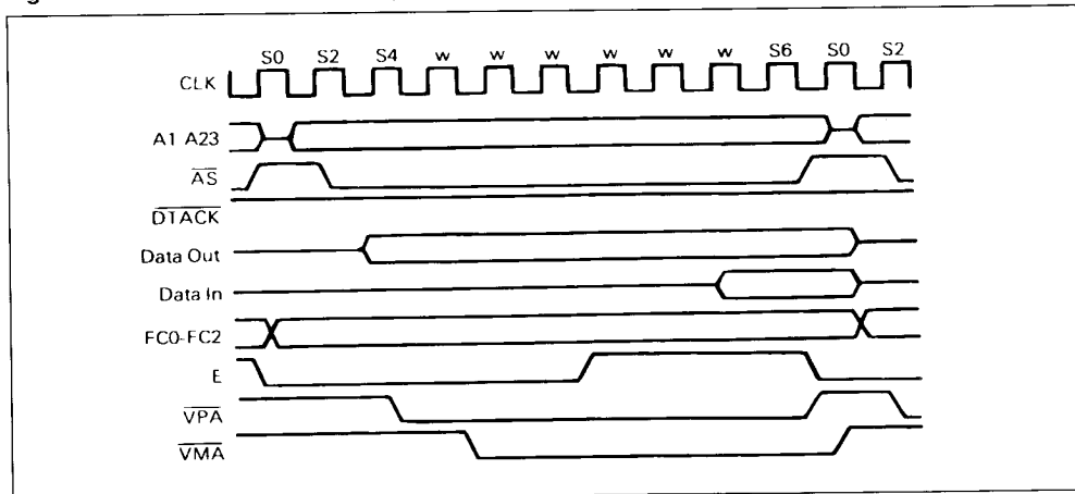
Figure 6.3 : TS68000 to EF6800 Peripheral Timing – Worst Case.
