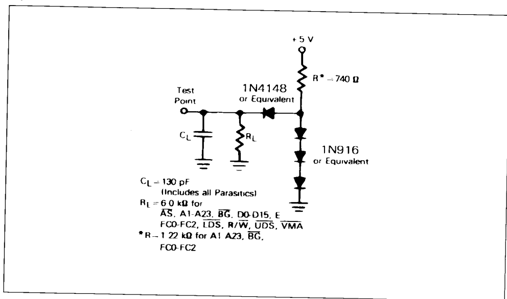
Figure 8.3 : Test Loads.
