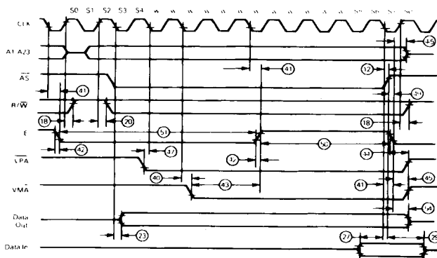
Figure 8.9 : TS68000 to 6800 Peripheral Timing Diagram – Best Case.
