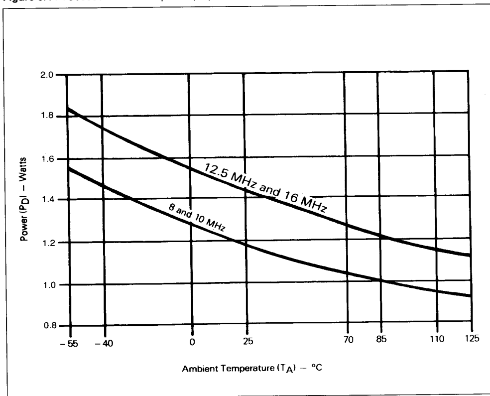
Figure 8.4 : TS68000 Power Dissipation ( P_D ) vs Ambient Temperature ( T_A ).
