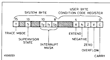
Figure 1.3 : Status Register.
