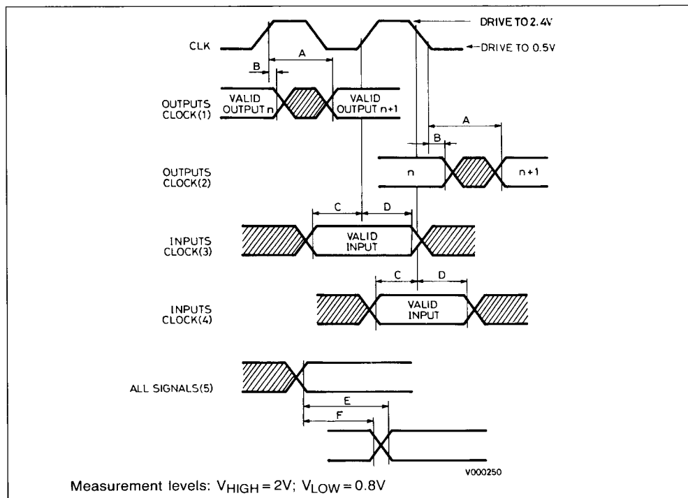
Figure 8.6 : Drive Levels and Test Points for AC Specifications.
