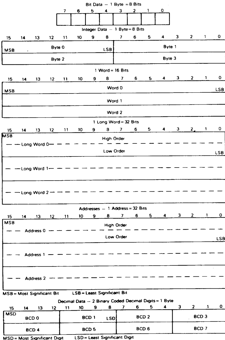
Figure 2.2 : Memory Data Organization.
