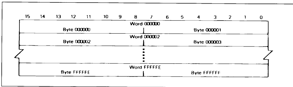
Figure 2.1 : Word Organization in Memory.
